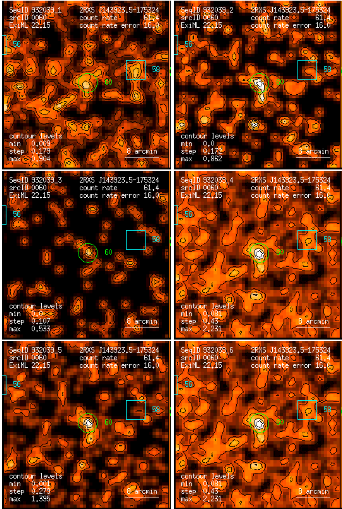
Figure 60: RASS 932039: detection 0060: band rate images, Gaussian filter: (1) PSPC channels 11 – 41, (2) 52 – 90, (3) 91 – 201, (4) 11 – 235, (5) 52 – 201, (6) 11 – 201. Broad band rates in counts/ks. Band rate contour levels in counts/ks/arcmin 2 .
