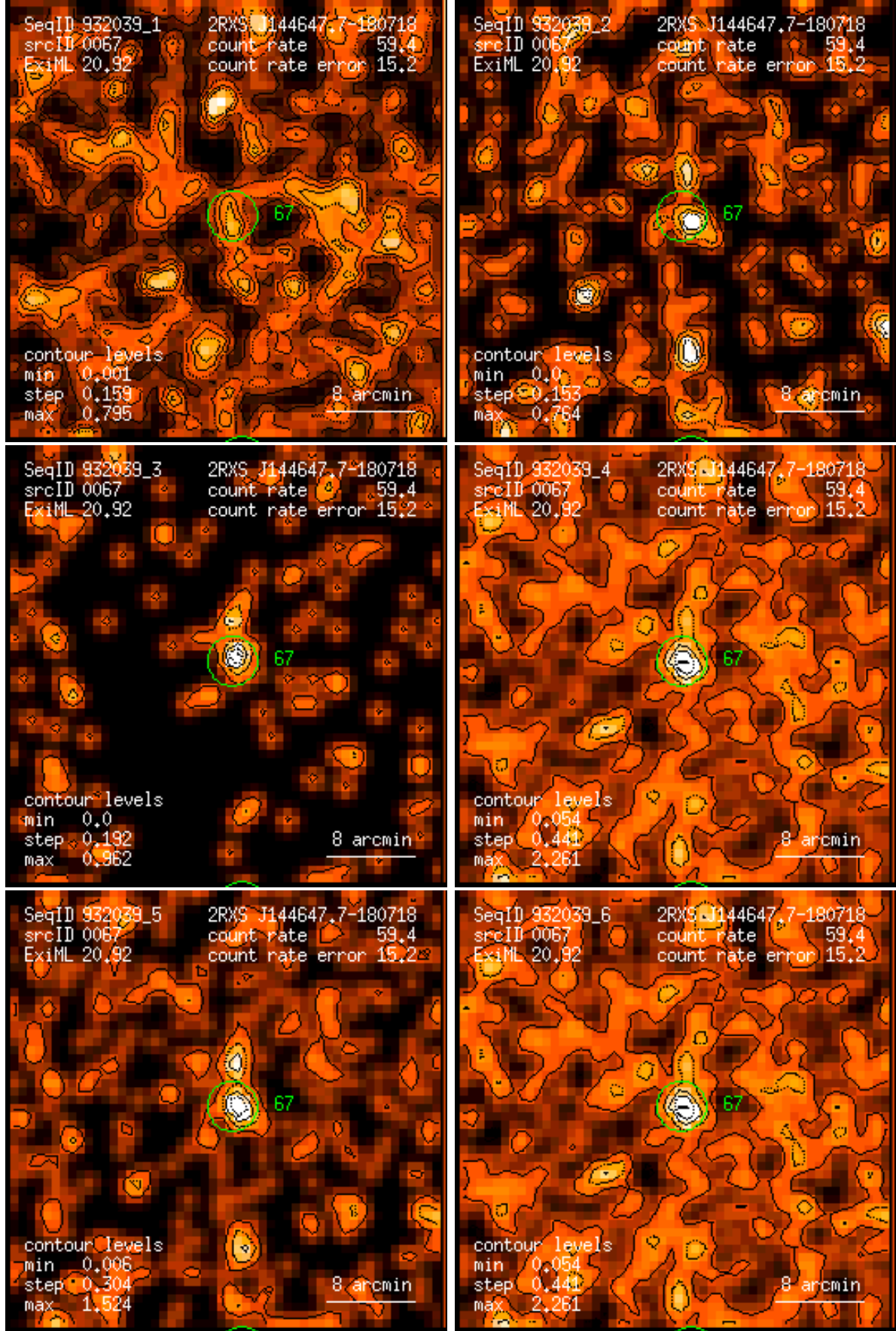
Figure 67: RASS 932039: detection 0067: band rate images, Gaussian filter: (1) PSPC channels 11 – 41, (2) 52 – 90, (3) 91 – 201, (4) 11 – 235, (5) 52 – 201, (6) 11 – 201. Broad band rates in counts/ks. Band rate contour levels in counts/ks/arcmin 2 .
