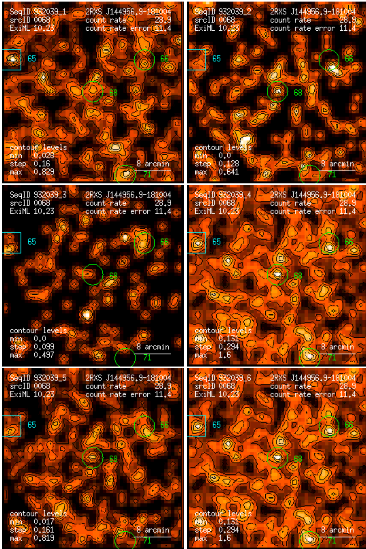
Figure 68: RASS 932039: detection 0068: band rate images, Gaussian filter: (1) PSPC channels 11 – 41, (2) 52 – 90, (3) 91 – 201, (4) 11 – 235, (5) 52 – 201, (6) 11 – 201. Broad band rates in counts/ks. Band rate contour levels in counts/ks/arcmin 2 .
