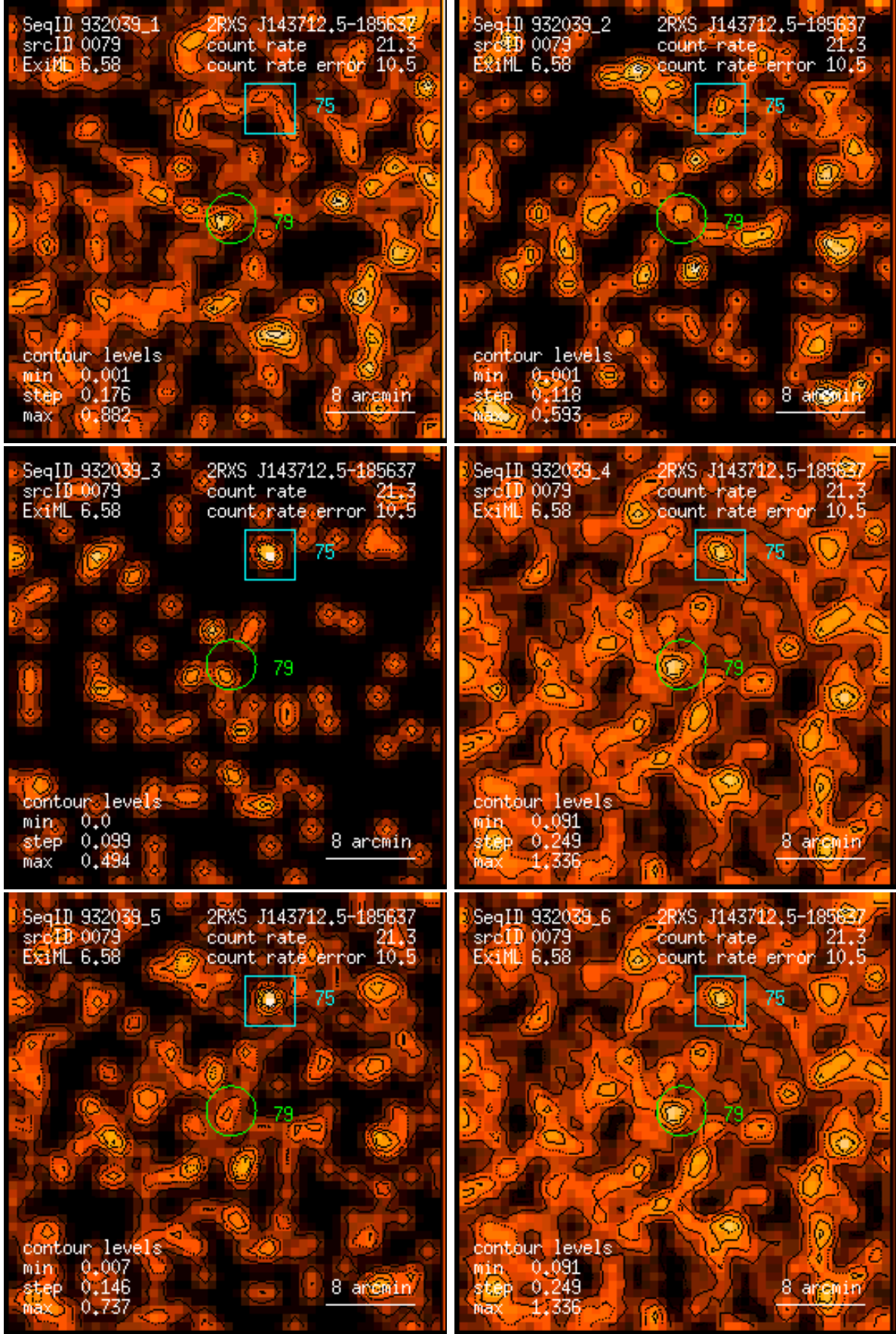
Figure 79: RASS 932039: detection 0079: band rate images, Gaussian filter: (1) PSPC channels 11 – 41, (2) 52 – 90, (3) 91 – 201, (4) 11 – 235, (5) 52 – 201, (6) 11 – 201. Broad band rates in counts/ks. Band rate contour levels in counts/ks/arcmin 2 .
