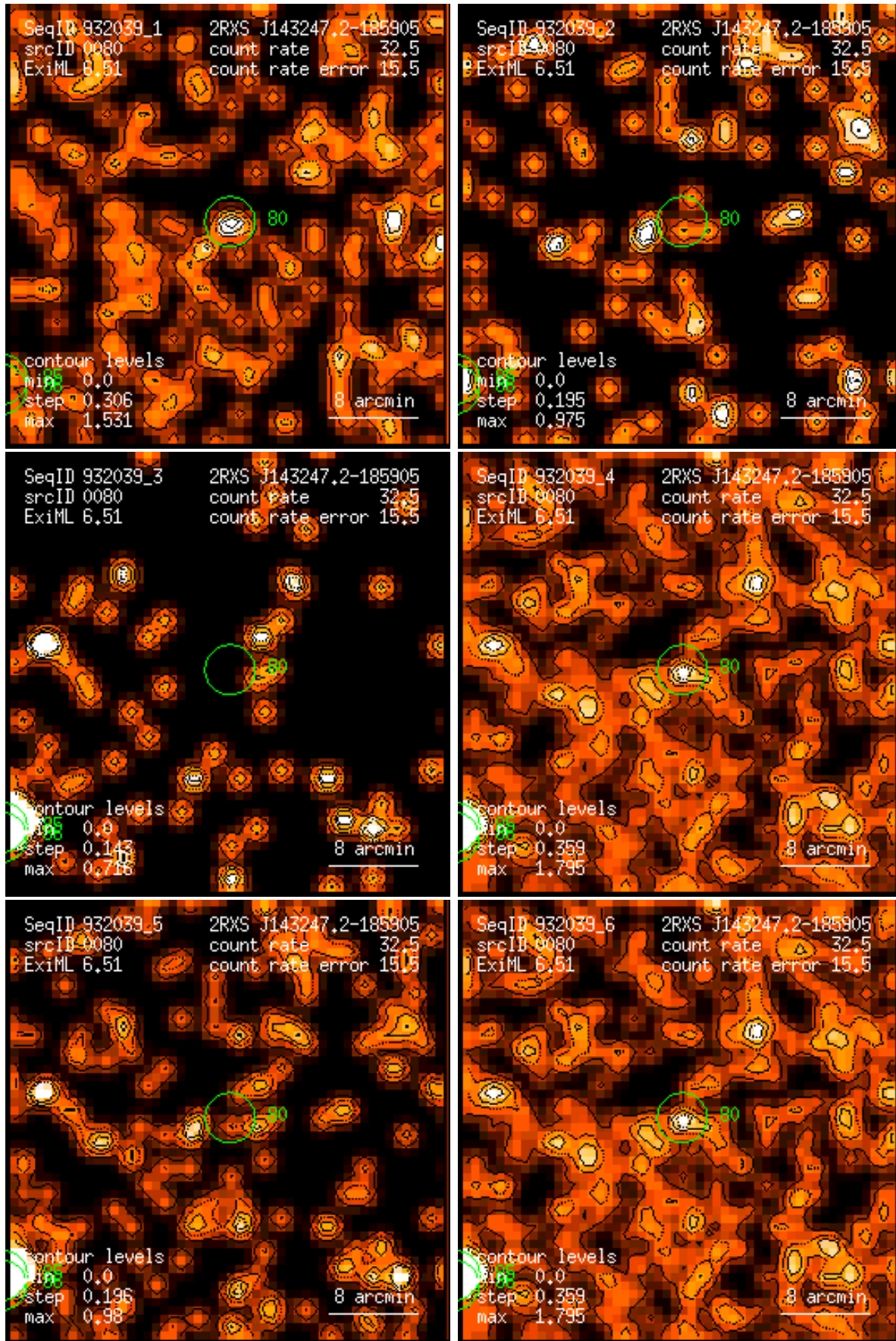
Figure 80: RASS 932039: detection 0080: band rate images, Gaussian filter: (1) PSPC channels 11 – 41, (2) 52 – 90, (3) 91 – 201, (4) 11 – 235, (5) 52 – 201, (6) 11 – 201. Broad band rates in counts/ks. Band rate contour levels in counts/ks/arcmin 2 .
