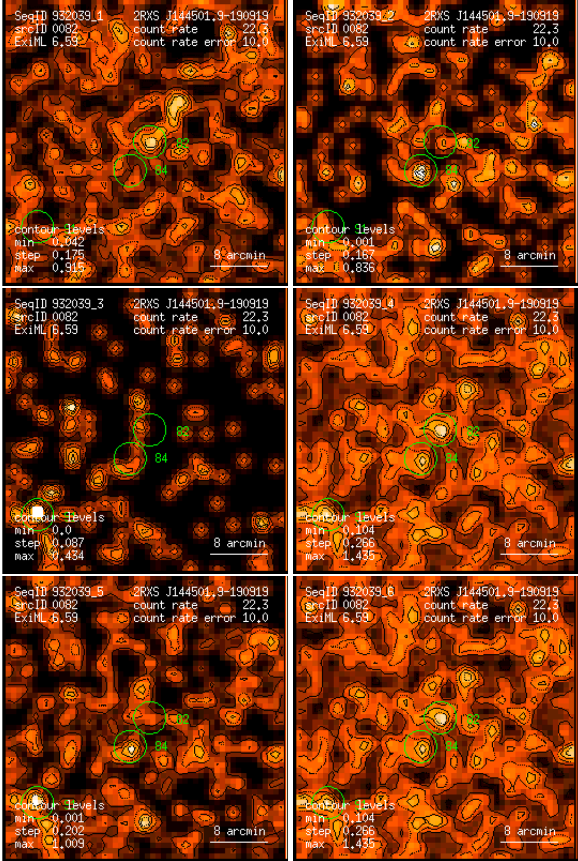
Figure 82: RASS 932039: detection 0082: band rate images, Gaussian filter: (1) PSPC channels 11 – 41, (2) 52 – 90, (3) 91 – 201, (4) 11 – 235, (5) 52 – 201, (6) 11 – 201. Broad band rates in counts/ks. Band rate contour levels in counts/ks/arcmin 2 .
