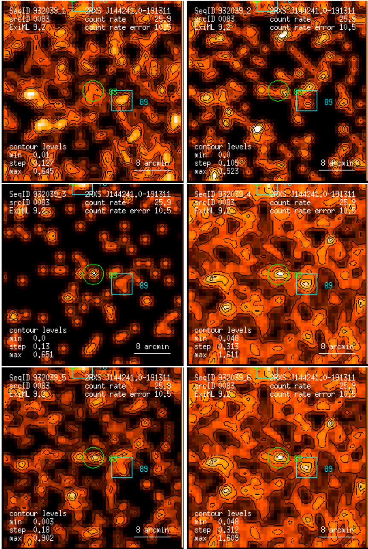
Figure 83: RASS 932039: detection 0083: band rate images, Gaussian filter: (1) PSPC channels 11 – 41, (2) 52 – 90, (3) 91 – 201, (4) 11 – 235, (5) 52 – 201, (6) 11 – 201. Broad band rates in counts/ks. Band rate contour levels in counts/ks/arcmin 2 .
