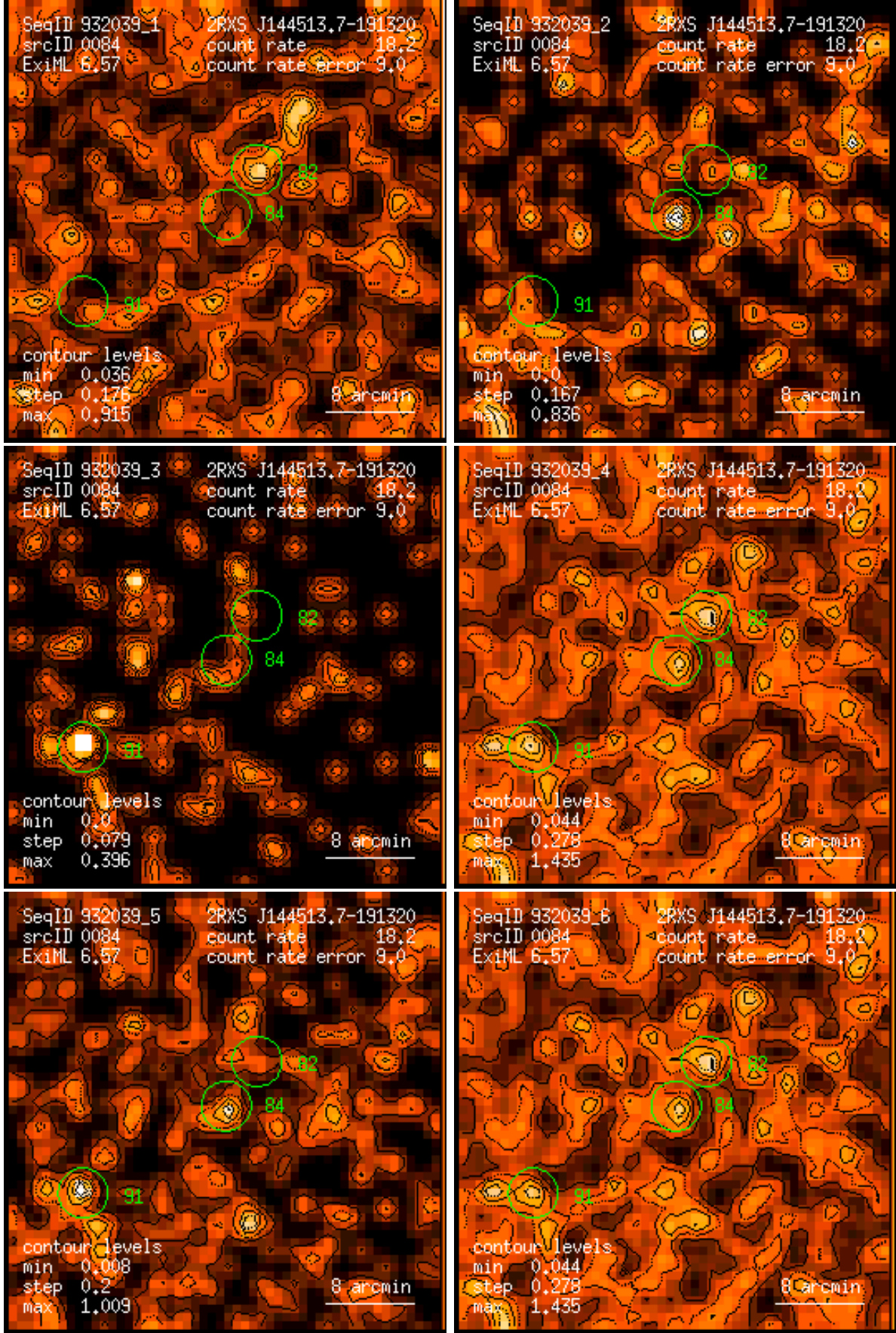
Figure 84: RASS 932039: detection 0084: band rate images, Gaussian filter: (1) PSPC channels 11 – 41, (2) 52 – 90, (3) 91 – 201, (4) 11 – 235, (5) 52 – 201, (6) 11 – 201. Broad band rates in counts/ks. Band rate contour levels in counts/ks/arcmin 2 .
