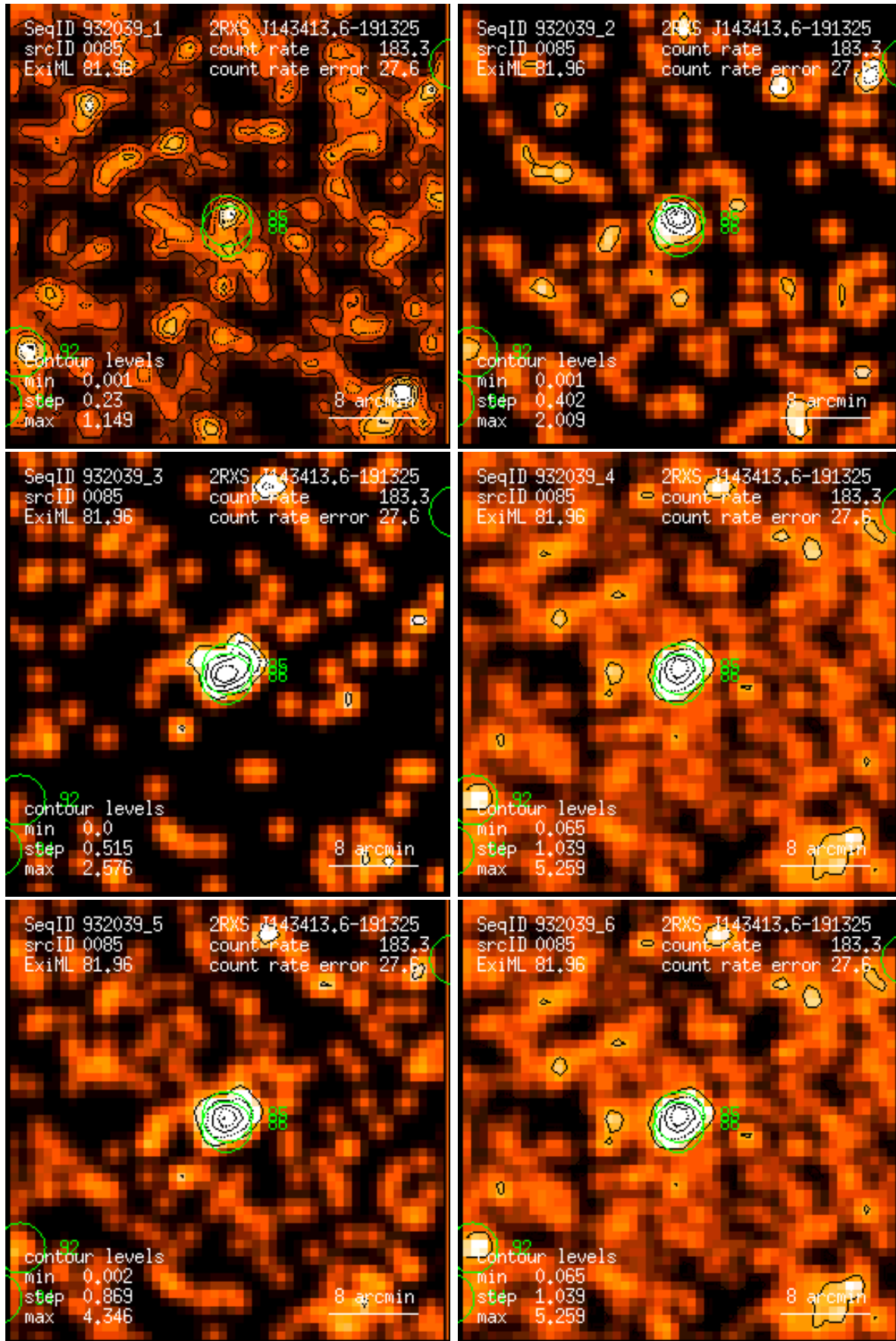
Figure 85: RASS 932039: detection 0085: band rate images, Gaussian filter: (1) PSPC channels 11 – 41, (2) 52 – 90, (3) 91 – 201, (4) 11 – 235, (5) 52 – 201, (6) 11 – 201. Broad band rates in counts/ks. Band rate contour levels in counts/ks/arcmin 2 .
