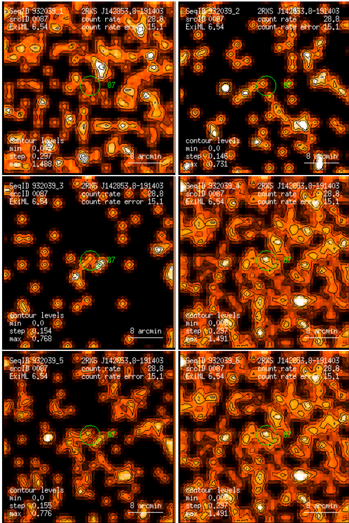
Figure 87: RASS 932039: detection 0087: band rate images, Gaussian filter: (1) PSPC channels 11 – 41, (2) 52 – 90, (3) 91 – 201, (4) 11 – 235, (5) 52 – 201, (6) 11 – 201. Broad band rates in counts/ks. Band rate contour levels in counts/ks/arcmin 2 .
