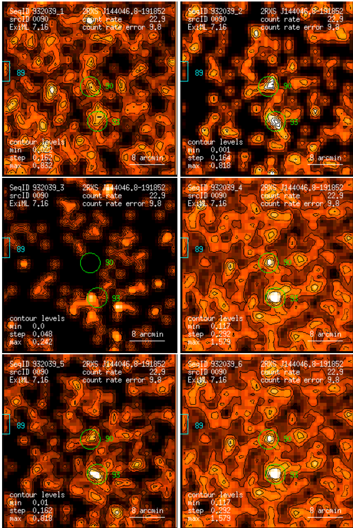
Figure 90: RASS 932039: detection 0090: band rate images, Gaussian filter: (1) PSPC channels 11 – 41, (2) 52 – 90, (3) 91 – 201, (4) 11 – 235, (5) 52 – 201, (6) 11 – 201. Broad band rates in counts/ks. Band rate contour levels in counts/ks/arcmin 2 .
