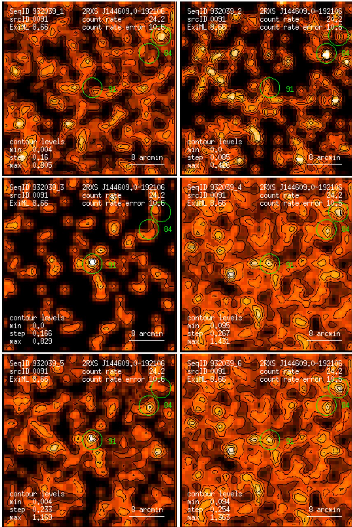
Figure 91: RASS 932039: detection 0091: band rate images, Gaussian filter: (1) PSPC channels 11 – 41, (2) 52 – 90, (3) 91 – 201, (4) 11 – 235, (5) 52 – 201, (6) 11 – 201. Broad band rates in counts/ks. Band rate contour levels in counts/ks/arcmin 2 .
