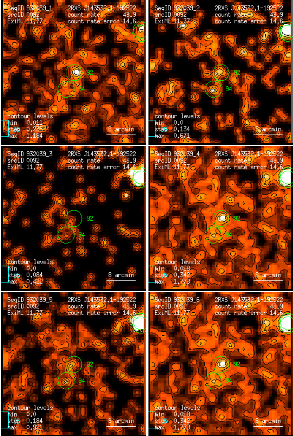
Figure 92: RASS 932039: detection 0092: band rate images, Gaussian filter: (1) PSPC channels 11 – 41, (2) 52 – 90, (3) 91 – 201, (4) 11 – 235, (5) 52 – 201, (6) 11 – 201. Broad band rates in counts/ks. Band rate contour levels in counts/ks/arcmin 2 .
