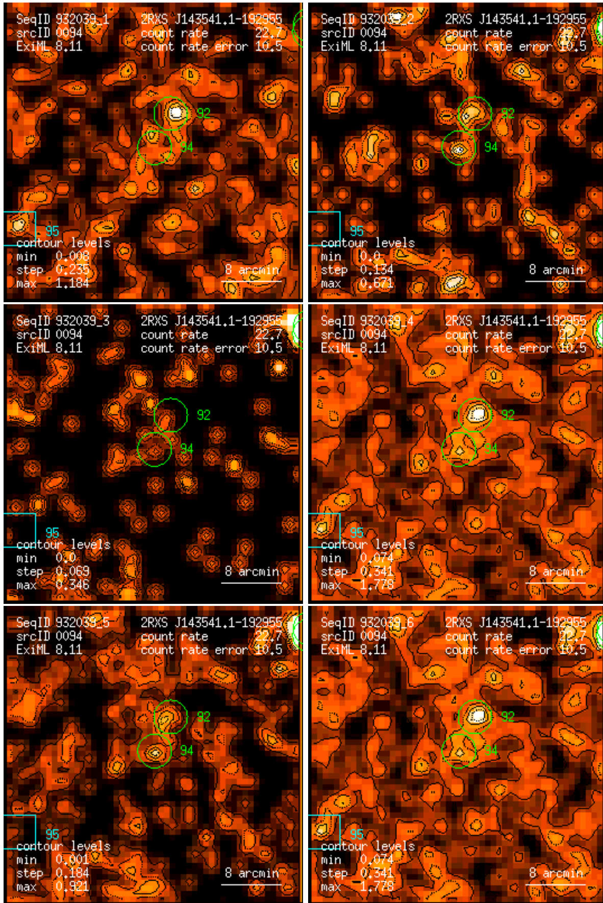
Figure 94: RASS 932039: detection 0094: band rate images, Gaussian filter: (1) PSPC channels 11 – 41, (2) 52 – 90, (3) 91 – 201, (4) 11 – 235, (5) 52 – 201, (6) 11 – 201. Broad band rates in counts/ks. Band rate contour levels in counts/ks/arcmin 2 .
