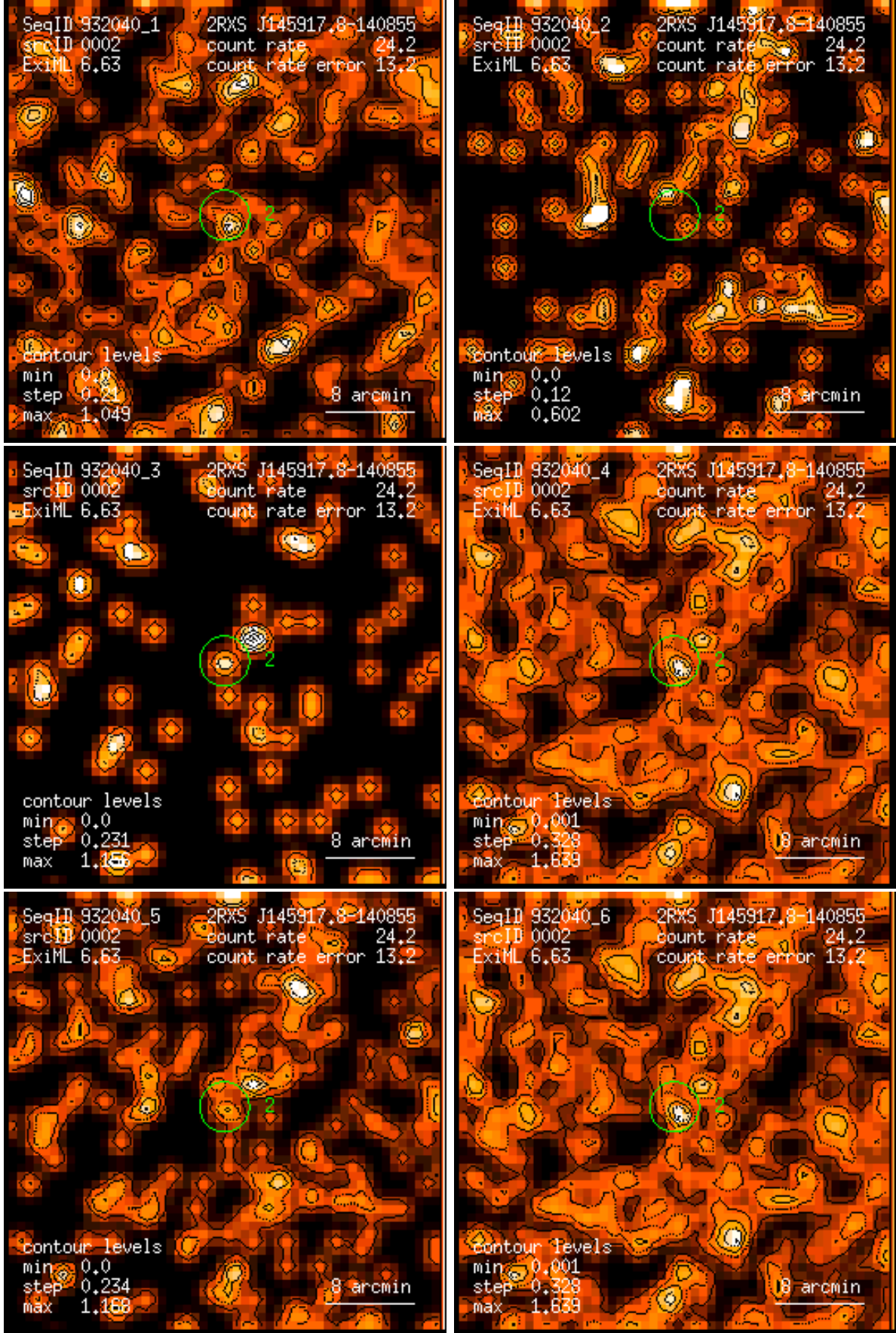
Figure 2: RASS 932040: detection 0002: band rate images, Gaussian filter: (1) PSPC channels 11 – 41, (2) 52 – 90, (3) 91 – 201, (4) 11 – 235, (5) 52 – 201, (6) 11 – 201. Broad band rates in counts/ks. Band rate contour levels in counts/ks/arcmin 2 .
