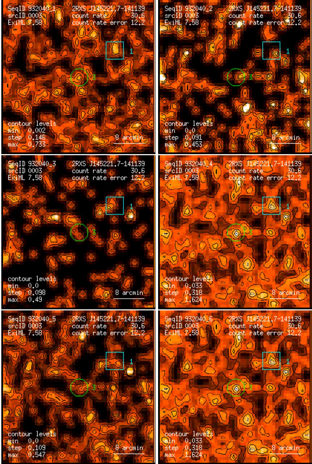
Figure 3: RASS 932040: detection 0003: band rate images, Gaussian filter: (1) PSPC channels 11 – 41, (2) 52 – 90, (3) 91 – 201, (4) 11 – 235, (5) 52 – 201, (6) 11 – 201. Broad band rates in counts/ks. Band rate contour levels in counts/ks/arcmin 2 .
