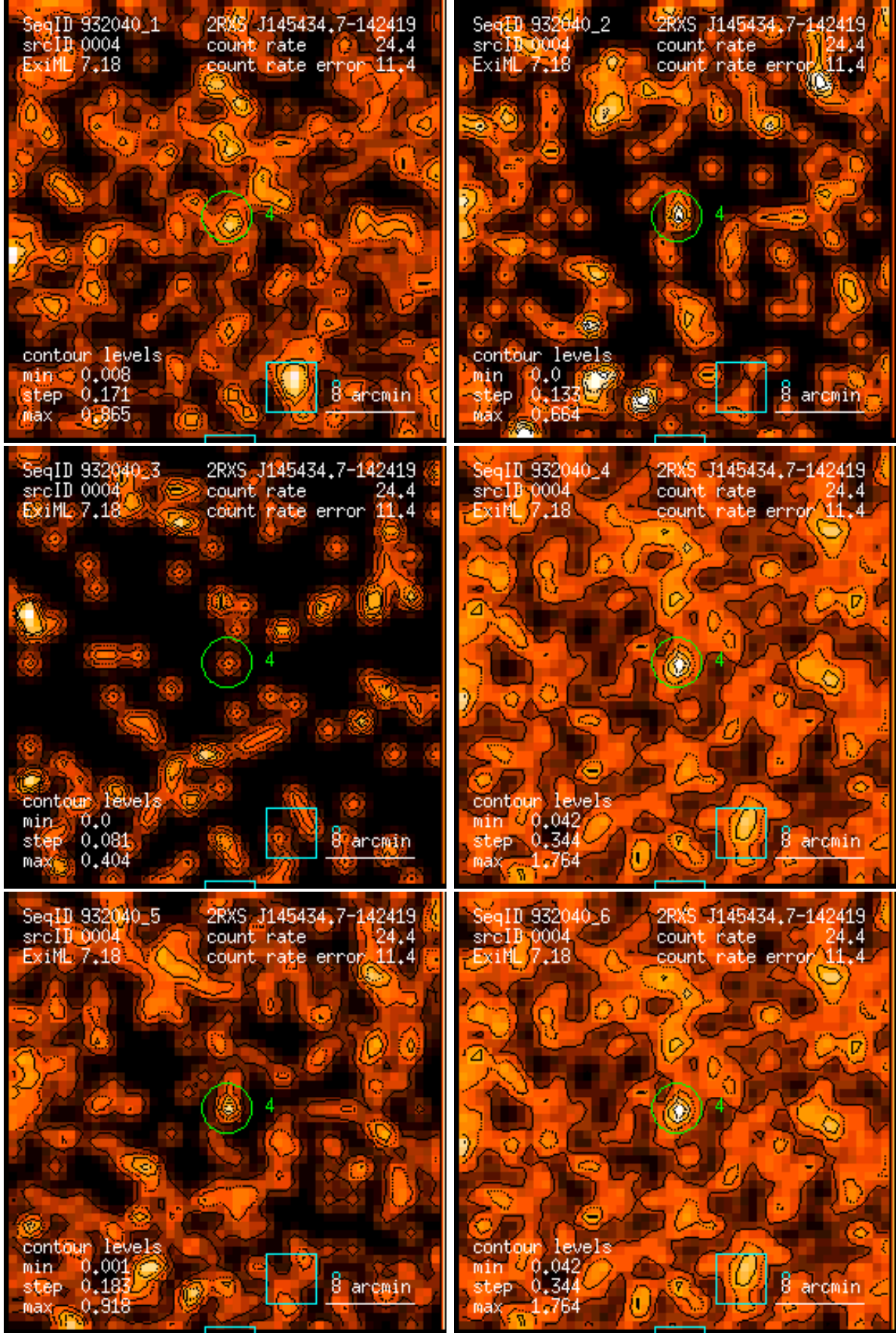
Figure 4: RASS 932040: detection 0004: band rate images, Gaussian filter: (1) PSPC channels 11 – 41, (2) 52 – 90, (3) 91 – 201, (4) 11 – 235, (5) 52 – 201, (6) 11 – 201. Broad band rates in counts/ks. Band rate contour levels in counts/ks/arcmin 2 .
