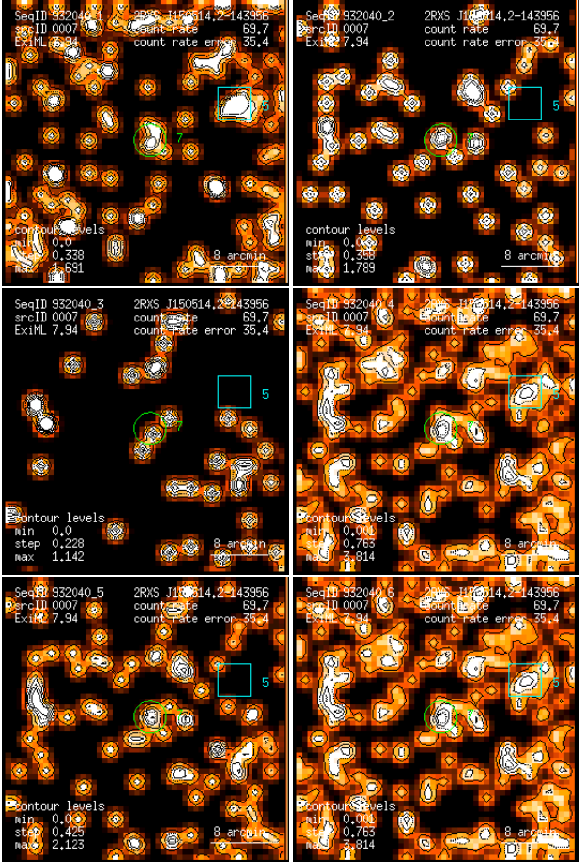
Figure 7: RASS 932040: detection 0007: band rate images, Gaussian filter: (1) PSPC channels 11 – 41, (2) 52 – 90, (3) 91 – 201, (4) 11 – 235, (5) 52 – 201, (6) 11 – 201. Broad band rates in counts/ks. Band rate contour levels in counts/ks/arcmin 2 .
