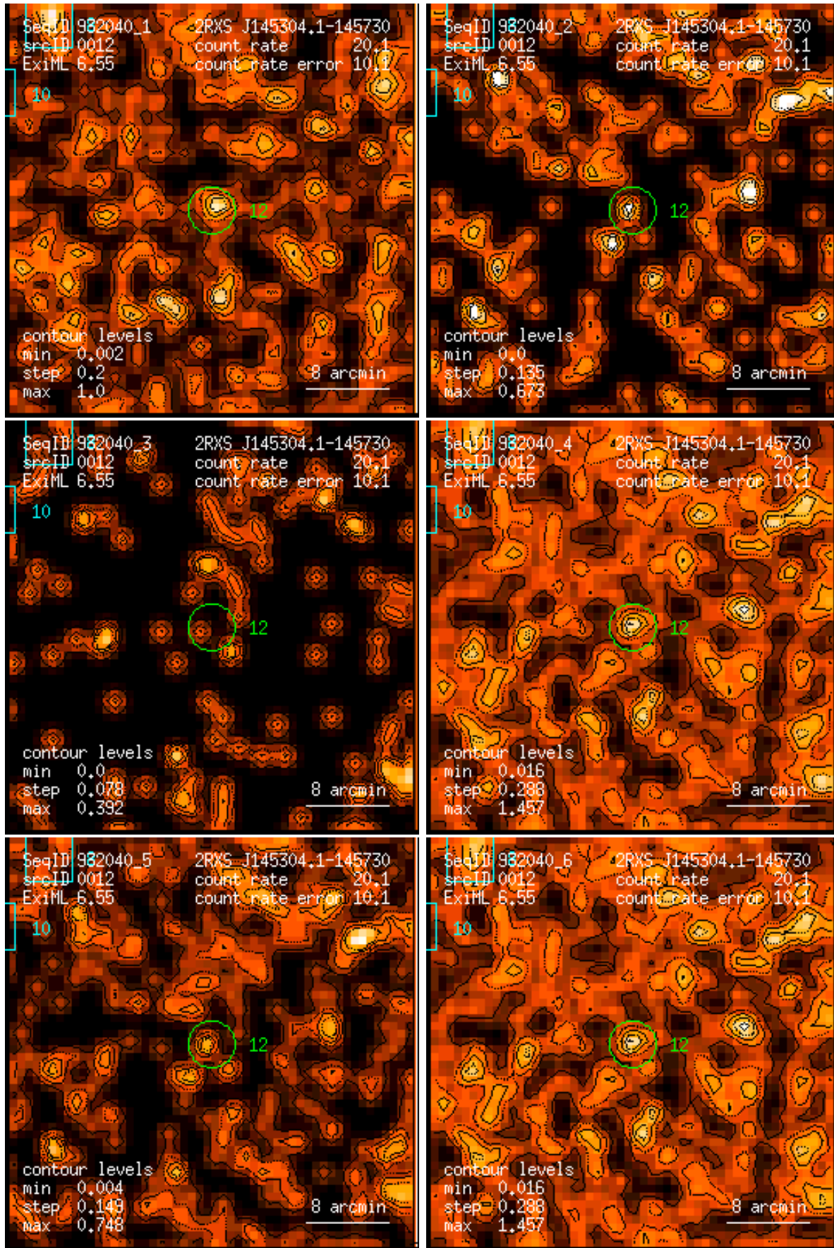
Figure 12: RASS 932040: detection 0012: band rate images, Gaussian filter: (1) PSPC channels 11 – 41, (2) 52 – 90, (3) 91 – 201, (4) 11 – 235, (5) 52 – 201, (6) 11 – 201. Broad band rates in counts/ks. Band rate contour levels in counts/ks/arcmin 2 .
