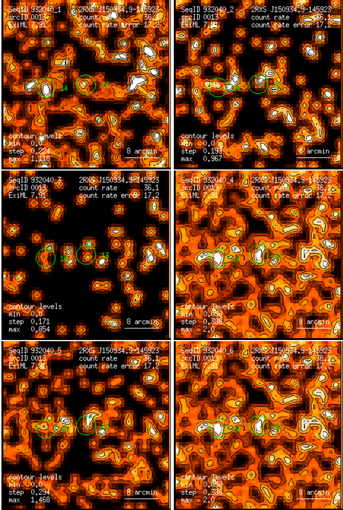
Figure 13: RASS 932040: detection 0013: band rate images, Gaussian filter: (1) PSPC channels 11 – 41, (2) 52 – 90, (3) 91 – 201, (4) 11 – 235, (5) 52 – 201, (6) 11 – 201. Broad band rates in counts/ks. Band rate contour levels in counts/ks/arcmin 2 .
