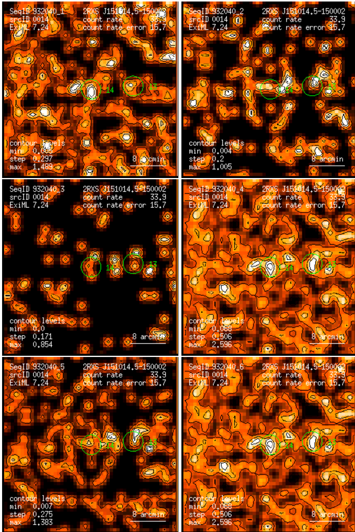
Figure 14: RASS 932040: detection 0014: band rate images, Gaussian filter: (1) PSPC channels 11 – 41, (2) 52 – 90, (3) 91 – 201, (4) 11 – 235, (5) 52 – 201, (6) 11 – 201. Broad band rates in counts/ks. Band rate contour levels in counts/ks/arcmin 2 .
