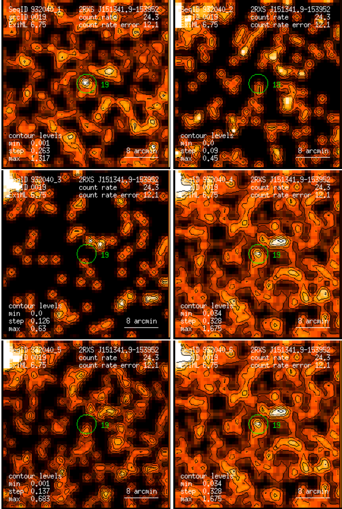
Figure 19: RASS 932040: detection 0019: band rate images, Gaussian filter: (1) PSPC channels 11 – 41, (2) 52 – 90, (3) 91 – 201, (4) 11 – 235, (5) 52 – 201, (6) 11 – 201. Broad band rates in counts/ks. Band rate contour levels in counts/ks/arcmin 2 .
