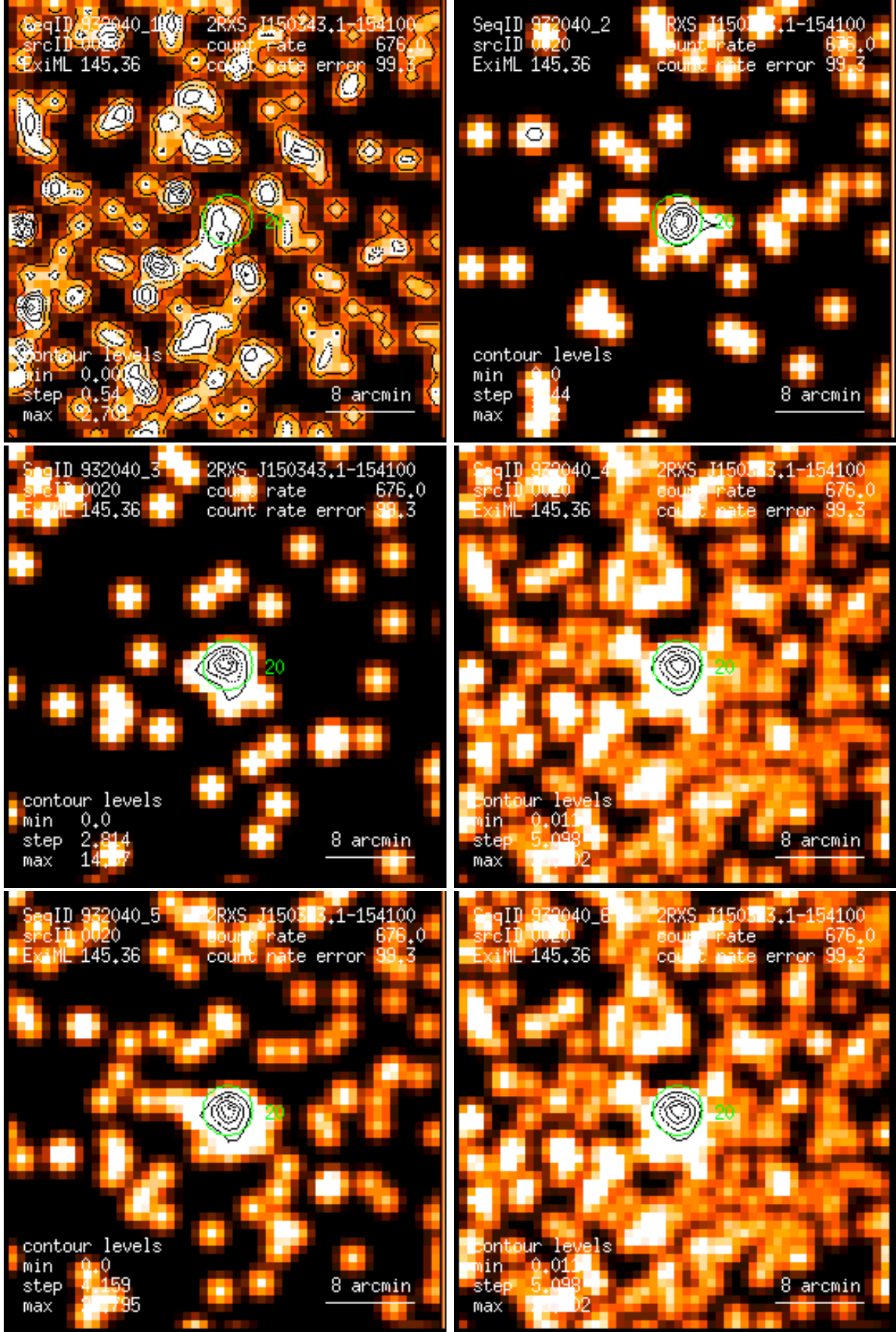
Figure 20: RASS 932040: detection 0020: band rate images, Gaussian filter: (1) PSPC channels 11 – 41, (2) 52 – 90, (3) 91 – 201, (4) 11 – 235, (5) 52 – 201, (6) 11 – 201. Broad band rates in counts/ks. Band rate contour levels in counts/ks/arcmin 2 .
