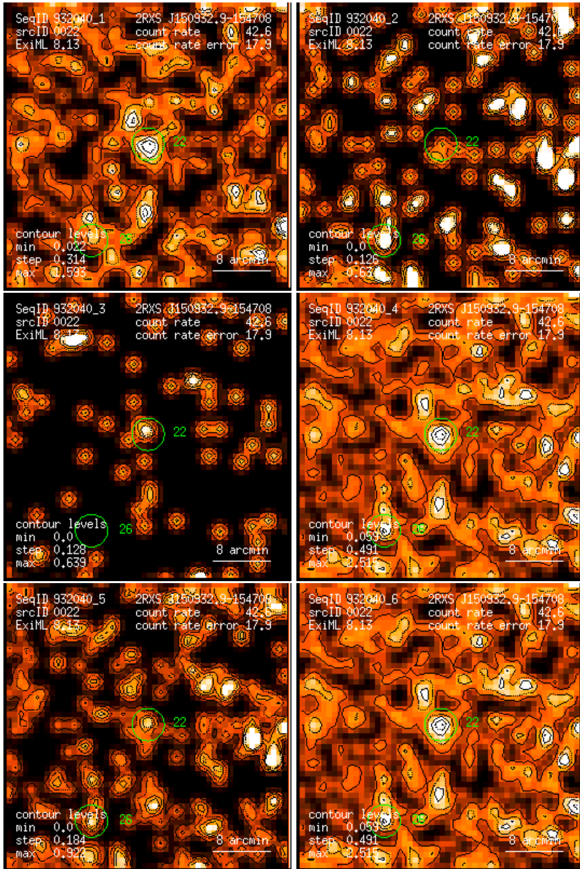
Figure 22: RASS 932040: detection 0022: band rate images, Gaussian filter: (1) PSPC channels 11 – 41, (2) 52 – 90, (3) 91 – 201, (4) 11 – 235, (5) 52 – 201, (6) 11 – 201. Broad band rates in counts/ks. Band rate contour levels in counts/ks/arcmin 2 .
