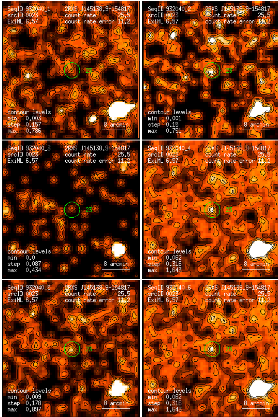
Figure 23: RASS 932040: detection 0023: band rate images, Gaussian filter: (1) PSPC channels 11 – 41, (2) 52 – 90, (3) 91 – 201, (4) 11 – 235, (5) 52 – 201, (6) 11 – 201. Broad band rates in counts/ks. Band rate contour levels in counts/ks/arcmin 2 .
