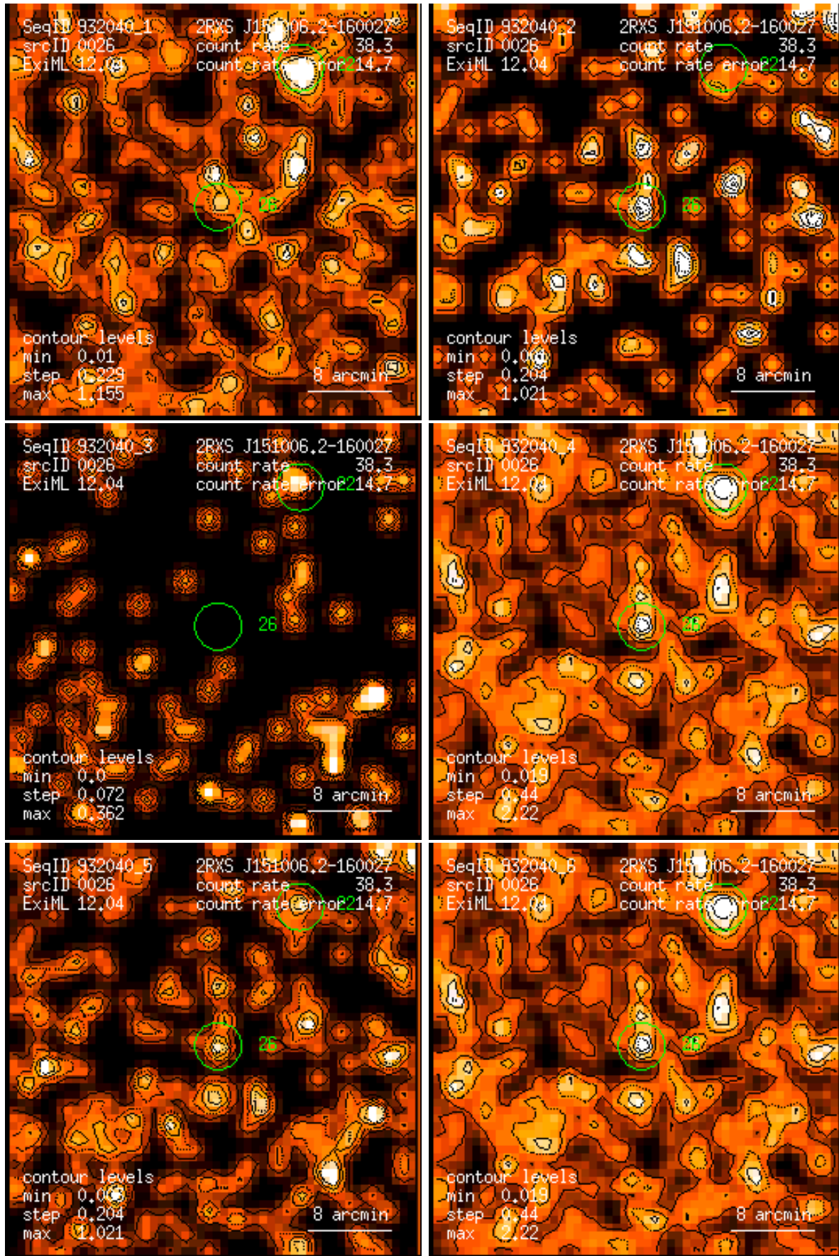
Figure 26: RASS 932040: detection 0026: band rate images, Gaussian filter: (1) PSPC channels 11 – 41, (2) 52 – 90, (3) 91 – 201, (4) 11 – 235, (5) 52 – 201, (6) 11 – 201. Broad band rates in counts/ks. Band rate contour levels in counts/ks/arcmin 2 .
