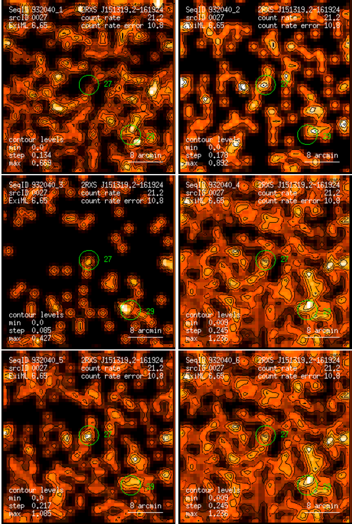
Figure 27: RASS 932040: detection 0027: band rate images, Gaussian filter: (1) PSPC channels 11 – 41, (2) 52 – 90, (3) 91 – 201, (4) 11 – 235, (5) 52 – 201, (6) 11 – 201. Broad band rates in counts/ks. Band rate contour levels in counts/ks/arcmin 2 .
