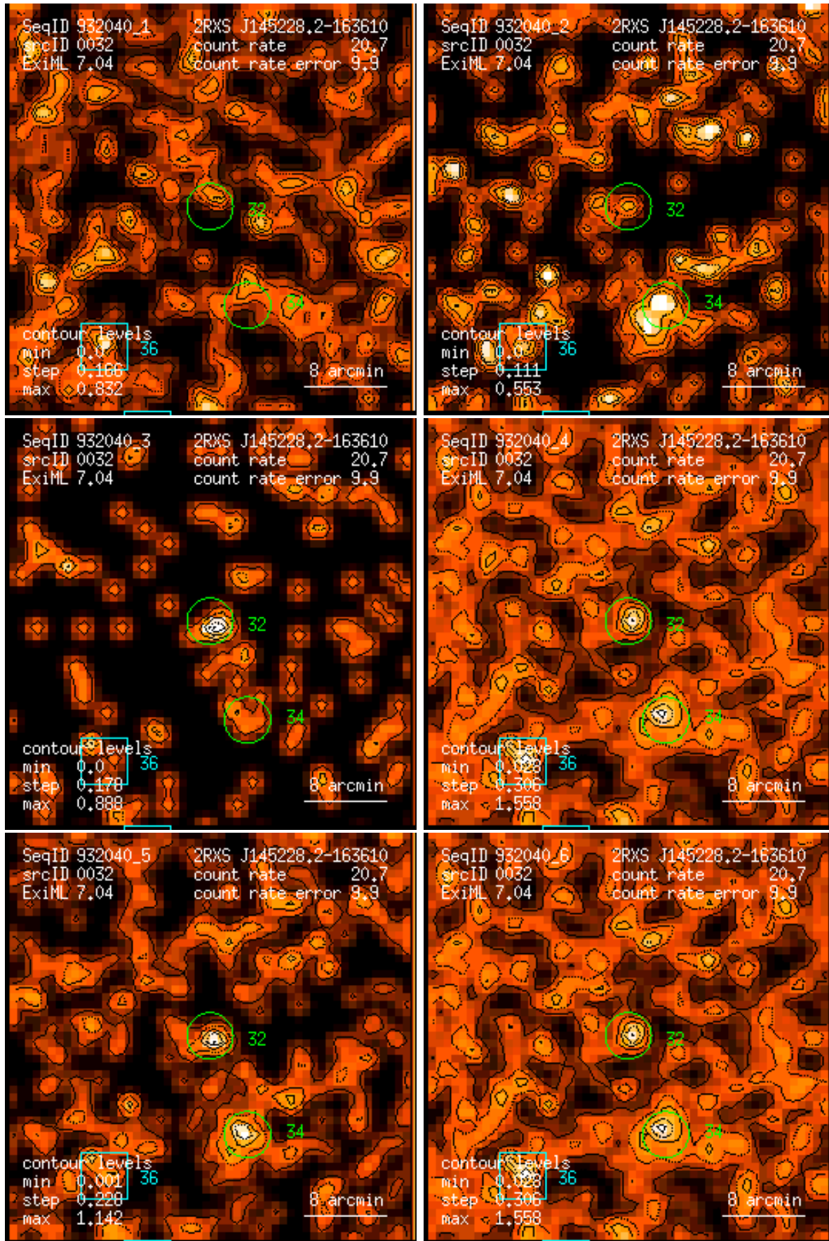
Figure 32: RASS 932040: detection 0032: band rate images, Gaussian filter: (1) PSPC channels 11 – 41, (2) 52 – 90, (3) 91 – 201, (4) 11 – 235, (5) 52 – 201, (6) 11 – 201. Broad band rates in counts/ks. Band rate contour levels in counts/ks/arcmin 2 .
