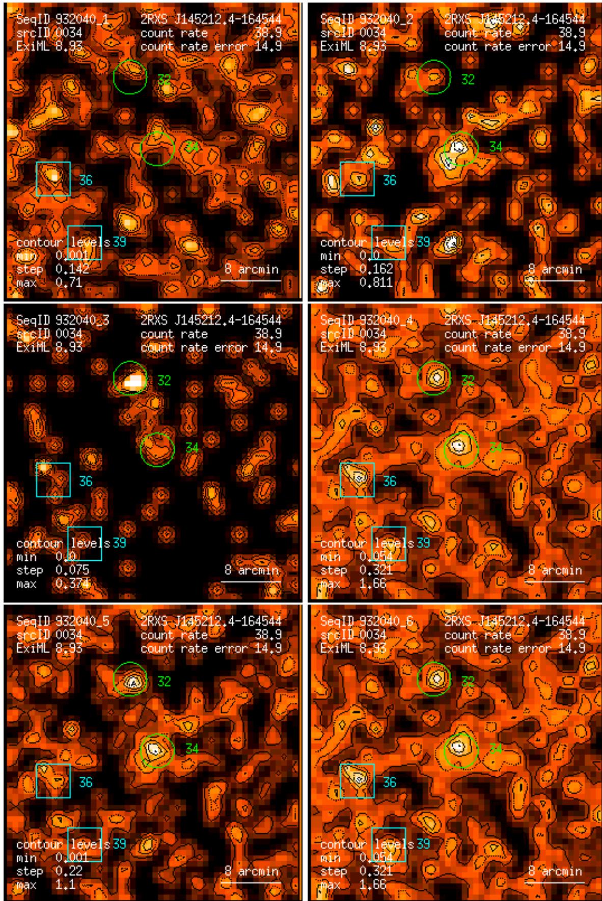
Figure 34: RASS 932040: detection 0034: band rate images, Gaussian filter: (1) PSPC channels 11 – 41, (2) 52 – 90, (3) 91 – 201, (4) 11 – 235, (5) 52 – 201, (6) 11 – 201. Broad band rates in counts/ks. Band rate contour levels in counts/ks/arcmin 2 .
