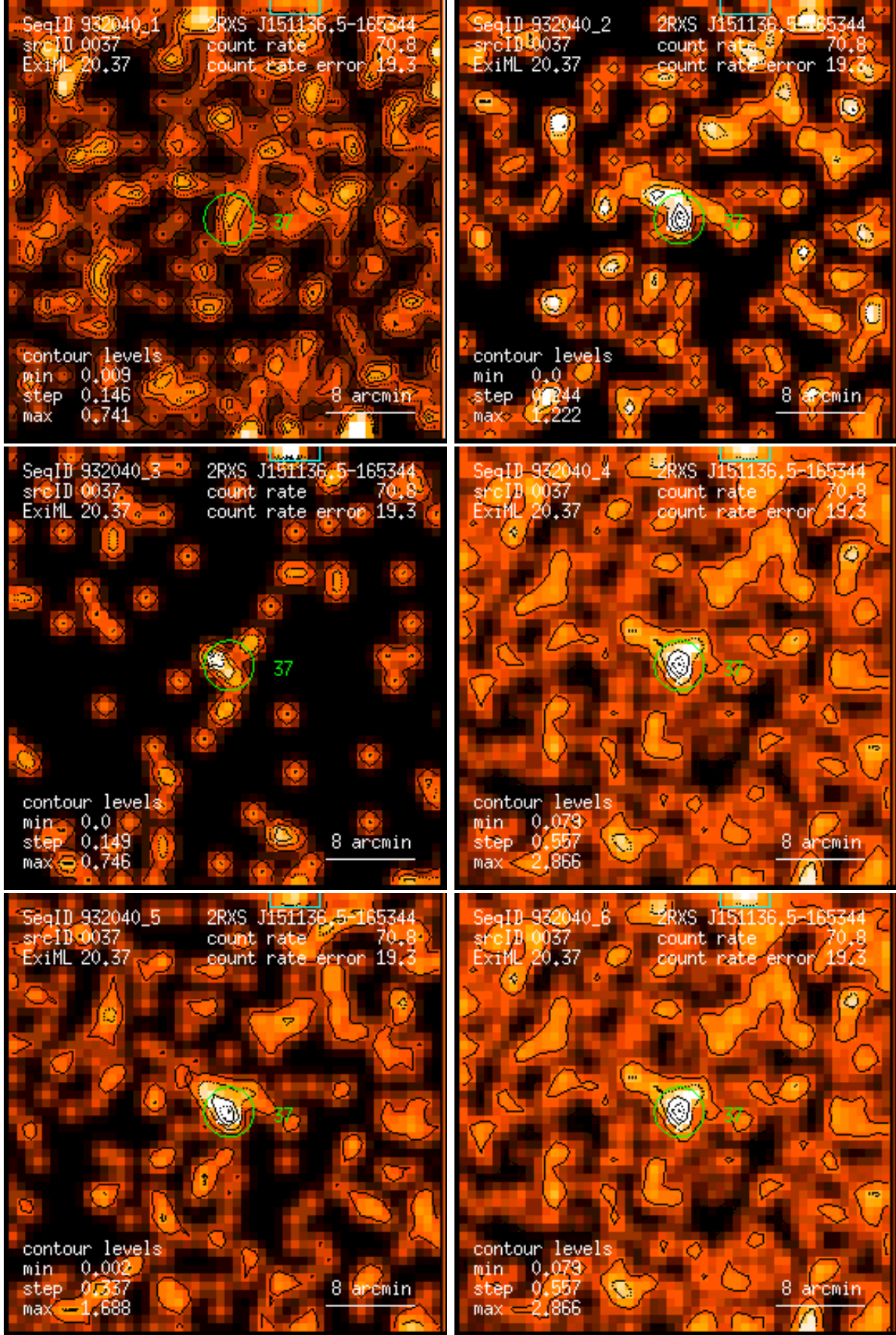
Figure 37: RASS 932040: detection 0037: band rate images, Gaussian filter: (1) PSPC channels 11 – 41, (2) 52 – 90, (3) 91 – 201, (4) 11 – 235, (5) 52 – 201, (6) 11 – 201. Broad band rates in counts/ks. Band rate contour levels in counts/ks/arcmin 2 .
