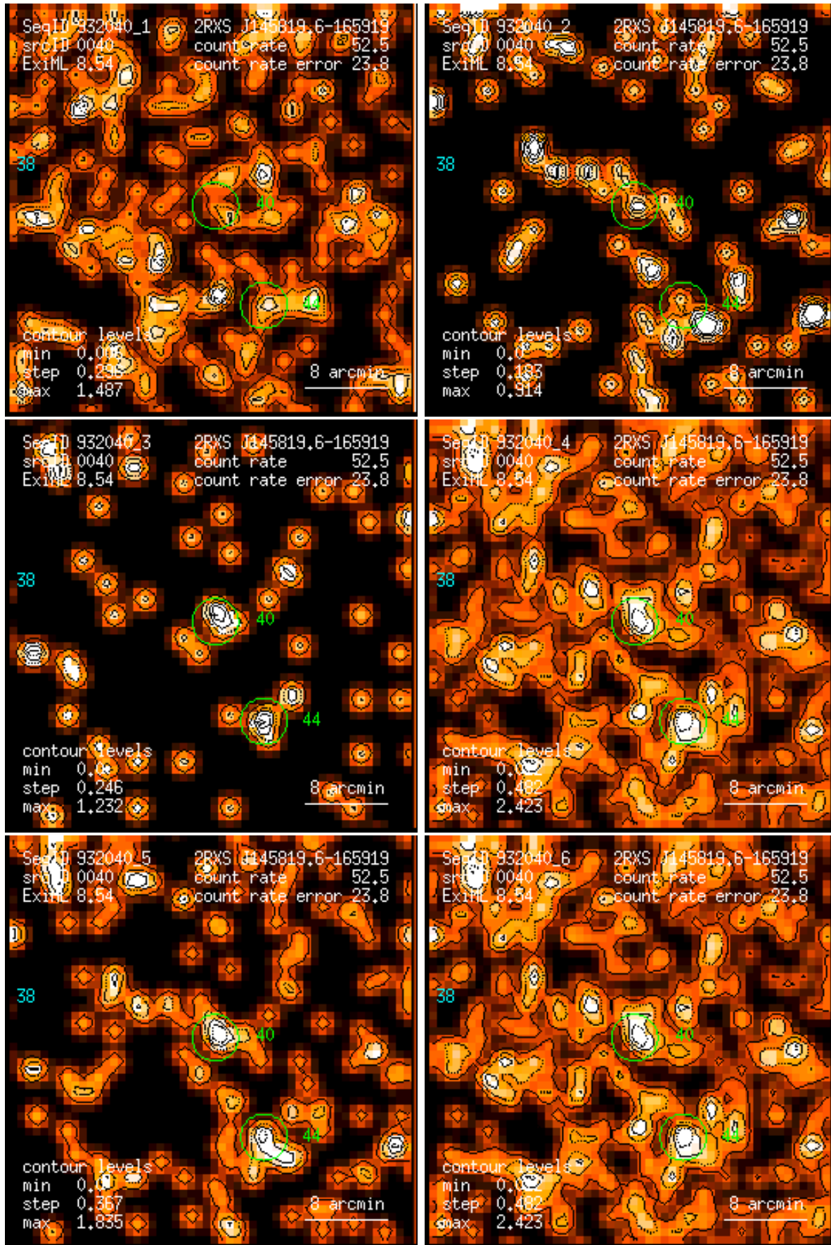
Figure 40: RASS 932040: detection 0040: band rate images, Gaussian filter: (1) PSPC channels 11 – 41, (2) 52 – 90, (3) 91 – 201, (4) 11 – 235, (5) 52 – 201, (6) 11 – 201. Broad band rates in counts/ks. Band rate contour levels in counts/ks/arcmin 2 .
