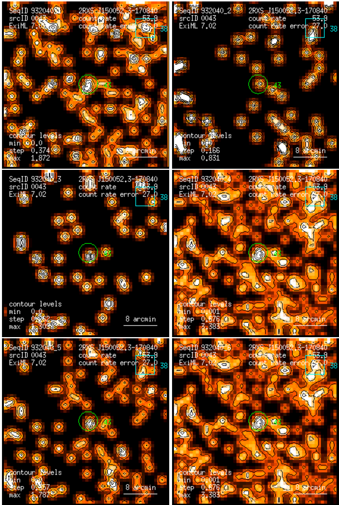
Figure 43: RASS 932040: detection 0043: band rate images, Gaussian filter: (1) PSPC channels 11 – 41, (2) 52 – 90, (3) 91 – 201, (4) 11 – 235, (5) 52 – 201, (6) 11 – 201. Broad band rates in counts/ks. Band rate contour levels in counts/ks/arcmin 2 .
