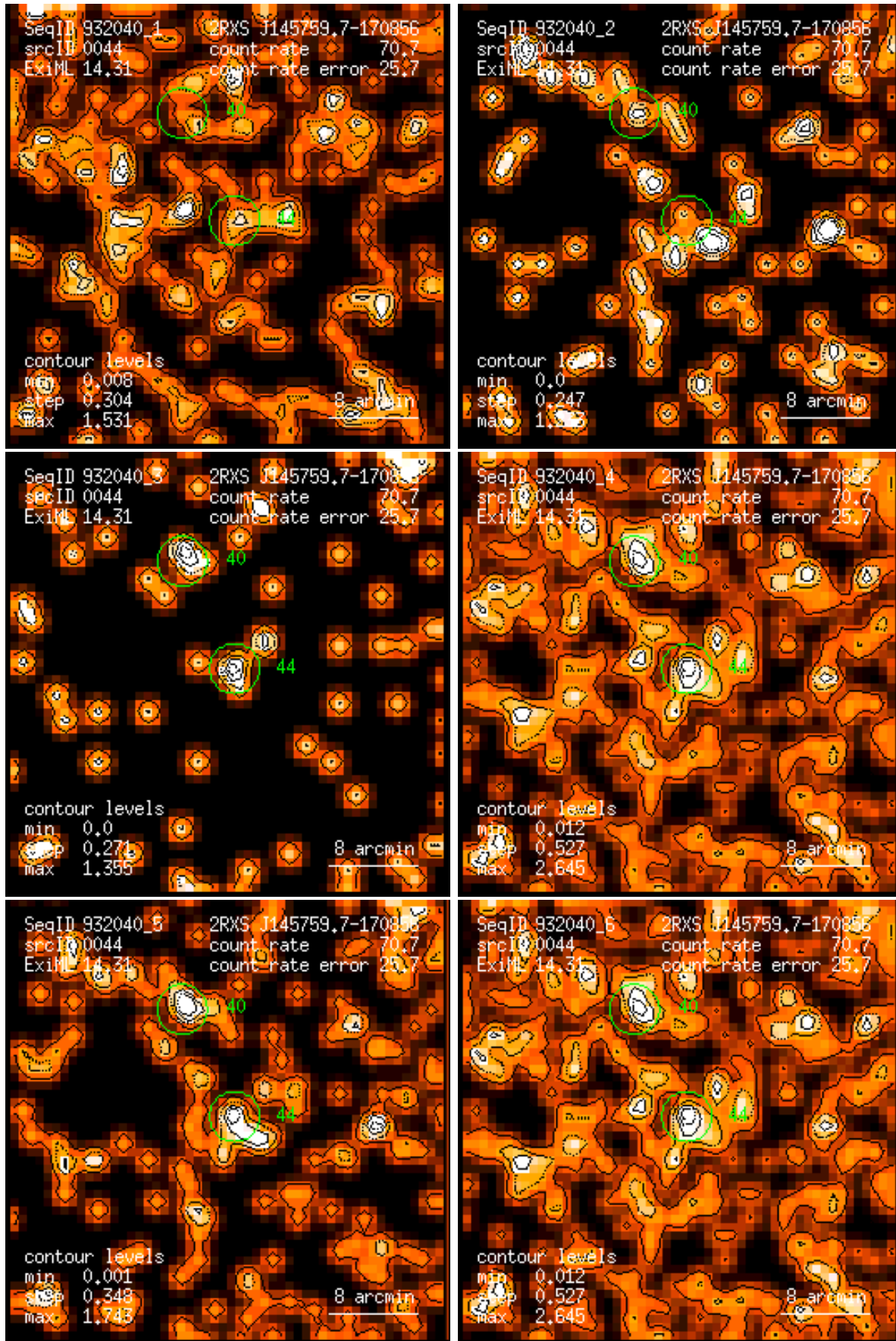
Figure 44: RASS 932040: detection 0044: band rate images, Gaussian filter: (1) PSPC channels 11 – 41, (2) 52 – 90, (3) 91 – 201, (4) 11 – 235, (5) 52 – 201, (6) 11 – 201. Broad band rates in counts/ks. Band rate contour levels in counts/ks/arcmin 2 .
