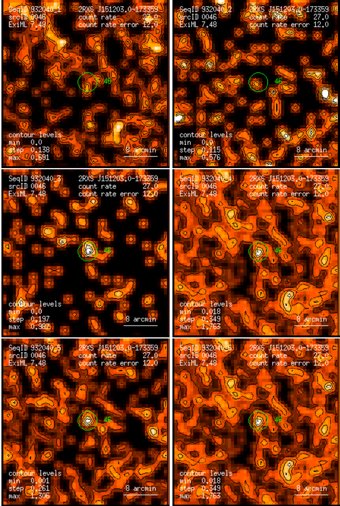
Figure 46: RASS 932040: detection 0046: band rate images, Gaussian filter: (1) PSPC channels 11 – 41, (2) 52 – 90, (3) 91 – 201, (4) 11 – 235, (5) 52 – 201, (6) 11 – 201. Broad band rates in counts/ks. Band rate contour levels in counts/ks/arcmin 2 .
