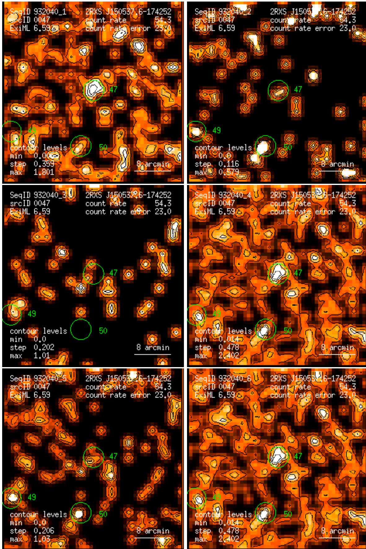
Figure 47: RASS 932040: detection 0047: band rate images, Gaussian filter: (1) PSPC channels 11 – 41, (2) 52 – 90, (3) 91 – 201, (4) 11 – 235, (5) 52 – 201, (6) 11 – 201. Broad band rates in counts/ks. Band rate contour levels in counts/ks/arcmin 2 .
