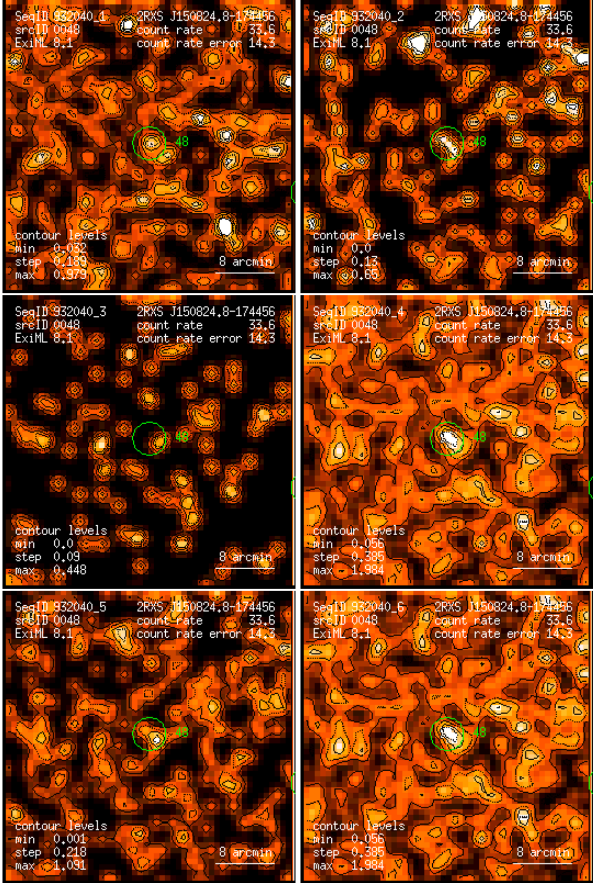
Figure 48: RASS 932040: detection 0048: band rate images, Gaussian filter: (1) PSPC channels 11 – 41, (2) 52 – 90, (3) 91 – 201, (4) 11 – 235, (5) 52 – 201, (6) 11 – 201. Broad band rates in counts/ks. Band rate contour levels in counts/ks/arcmin 2 .
