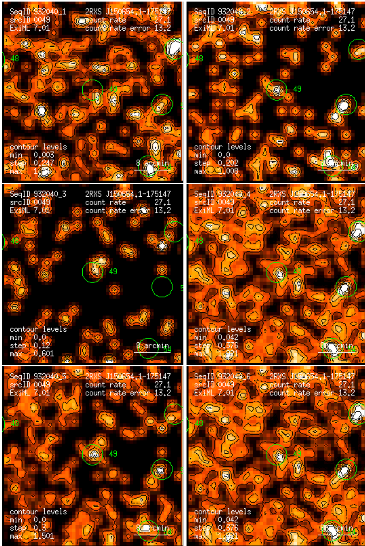
Figure 49: RASS 932040: detection 0049: band rate images, Gaussian filter: (1) PSPC channels 11 – 41, (2) 52 – 90, (3) 91 – 201, (4) 11 – 235, (5) 52 – 201, (6) 11 – 201. Broad band rates in counts/ks. Band rate contour levels in counts/ks/arcmin 2 .
