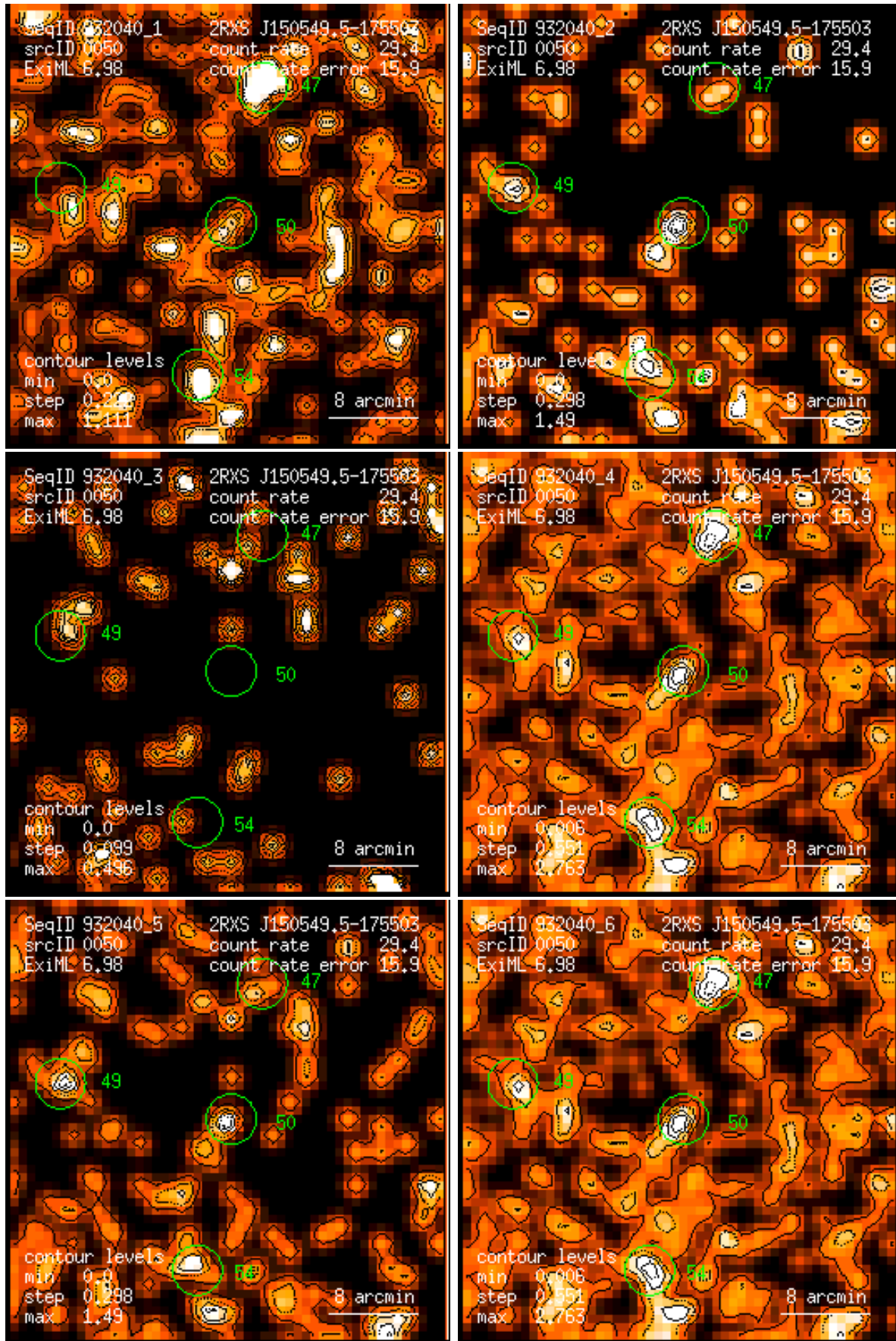
Figure 50: RASS 932040: detection 0050: band rate images, Gaussian filter: (1) PSPC channels 11 – 41, (2) 52 – 90, (3) 91 – 201, (4) 11 – 235, (5) 52 – 201, (6) 11 – 201. Broad band rates in counts/ks. Band rate contour levels in counts/ks/arcmin 2 .
