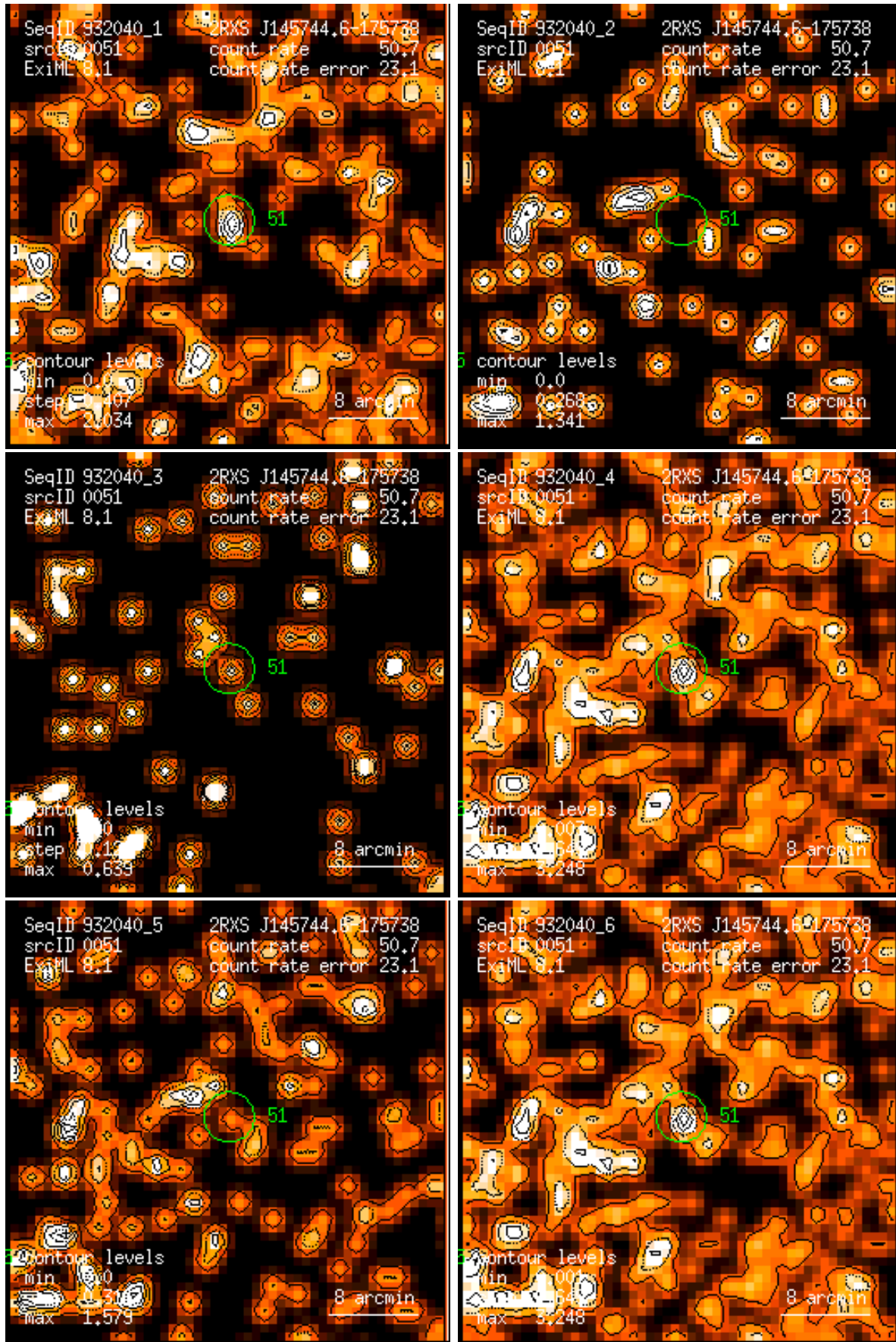
Figure 51: RASS 932040: detection 0051: band rate images, Gaussian filter: (1) PSPC channels 11 – 41, (2) 52 – 90, (3) 91 – 201, (4) 11 – 235, (5) 52 – 201, (6) 11 – 201. Broad band rates in counts/ks. Band rate contour levels in counts/ks/arcmin 2 .
