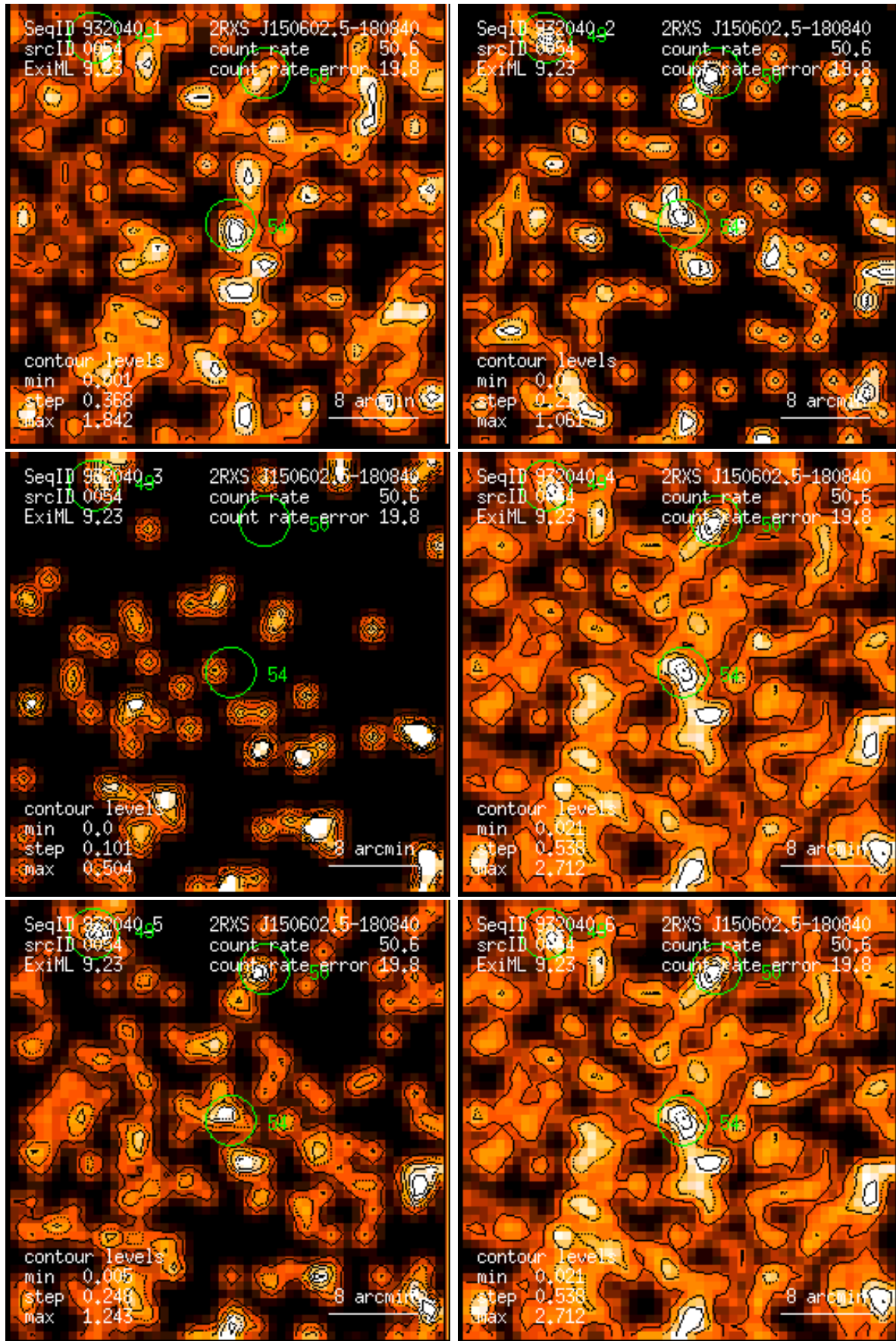
Figure 54: RASS 932040: detection 0054: band rate images, Gaussian filter: (1) PSPC channels 11 – 41, (2) 52 – 90, (3) 91 – 201, (4) 11 – 235, (5) 52 – 201, (6) 11 – 201. Broad band rates in counts/ks. Band rate contour levels in counts/ks/arcmin 2 .
