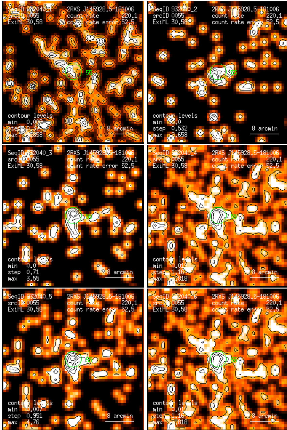
Figure 55: RASS 932040: detection 0055: band rate images, Gaussian filter: (1) PSPC channels 11 – 41, (2) 52 – 90, (3) 91 – 201, (4) 11 – 235, (5) 52 – 201, (6) 11 – 201. Broad band rates in counts/ks. Band rate contour levels in counts/ks/arcmin 2 .
