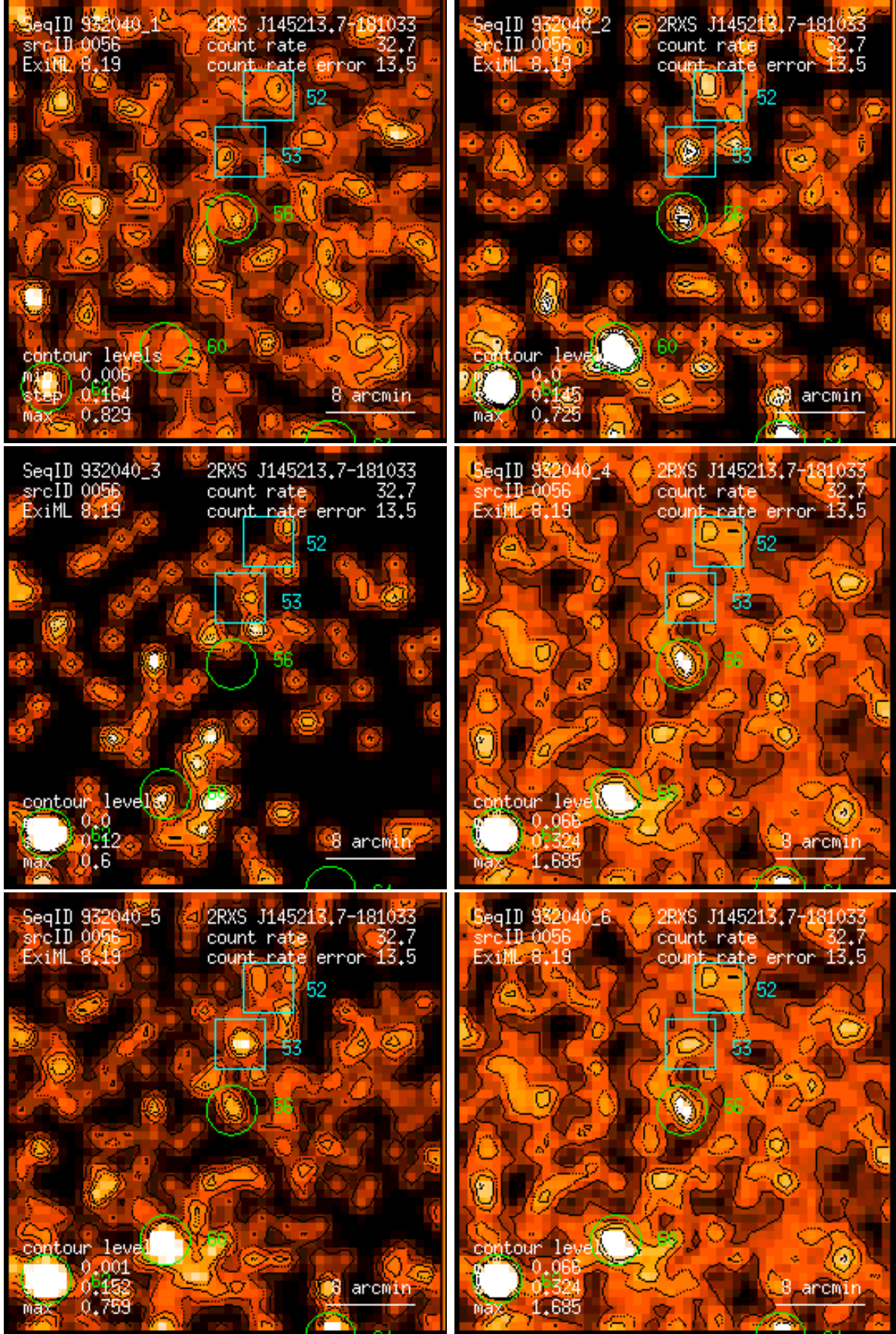
Figure 56: RASS 932040: detection 0056: band rate images, Gaussian filter: (1) PSPC channels 11 – 41, (2) 52 – 90, (3) 91 – 201, (4) 11 – 235, (5) 52 – 201, (6) 11 – 201. Broad band rates in counts/ks. Band rate contour levels in counts/ks/arcmin 2 .
