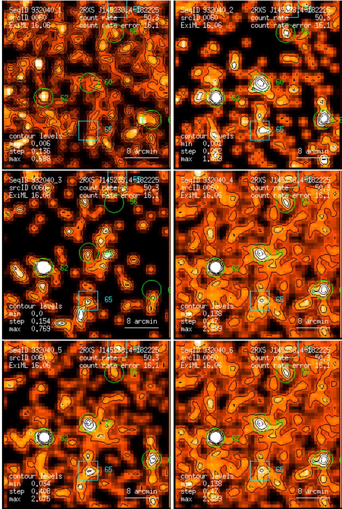
Figure 60: RASS 932040: detection 0060: band rate images, Gaussian filter: (1) PSPC channels 11 – 41, (2) 52 – 90, (3) 91 – 201, (4) 11 – 235, (5) 52 – 201, (6) 11 – 201. Broad band rates in counts/ks. Band rate contour levels in counts/ks/arcmin 2 .
