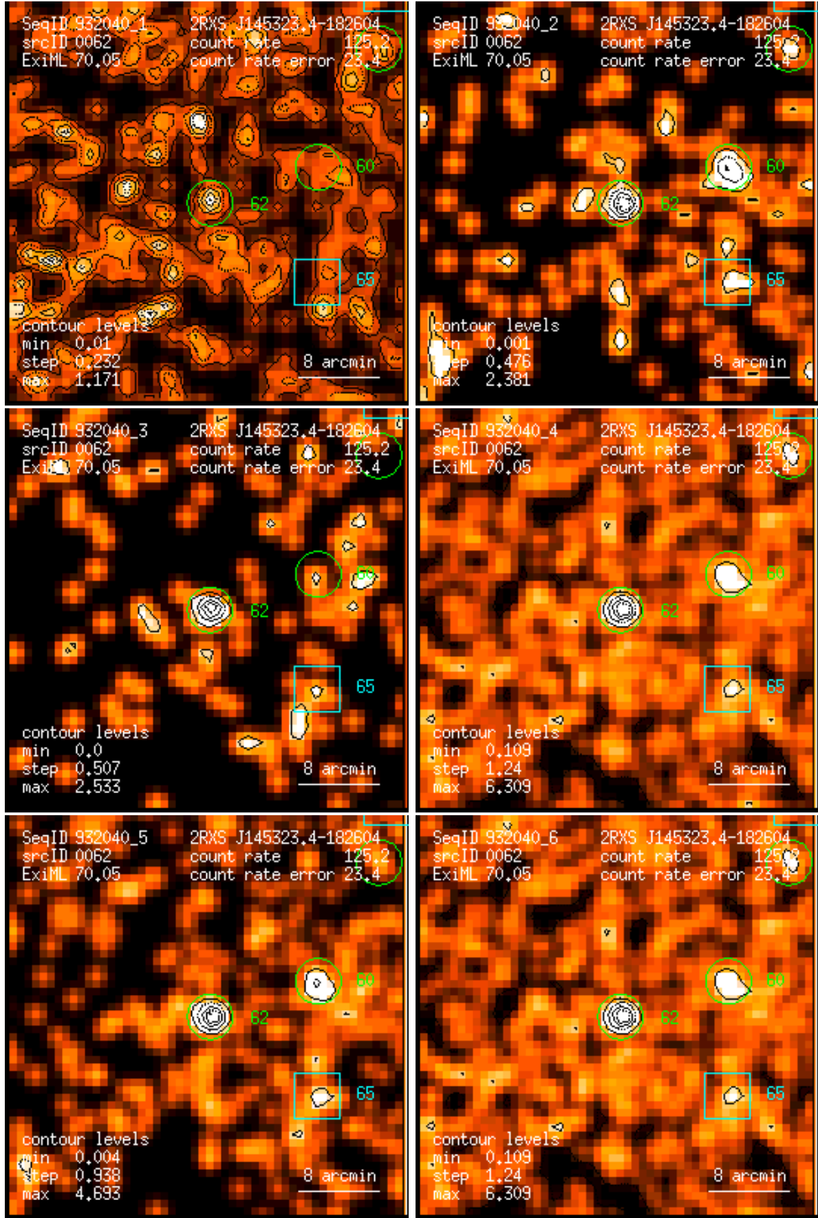
Figure 62: RASS 932040: detection 0062: band rate images, Gaussian filter: (1) PSPC channels 11 – 41, (2) 52 – 90, (3) 91 – 201, (4) 11 – 235, (5) 52 – 201, (6) 11 – 201. Broad band rates in counts/ks. Band rate contour levels in counts/ks/arcmin 2 .
