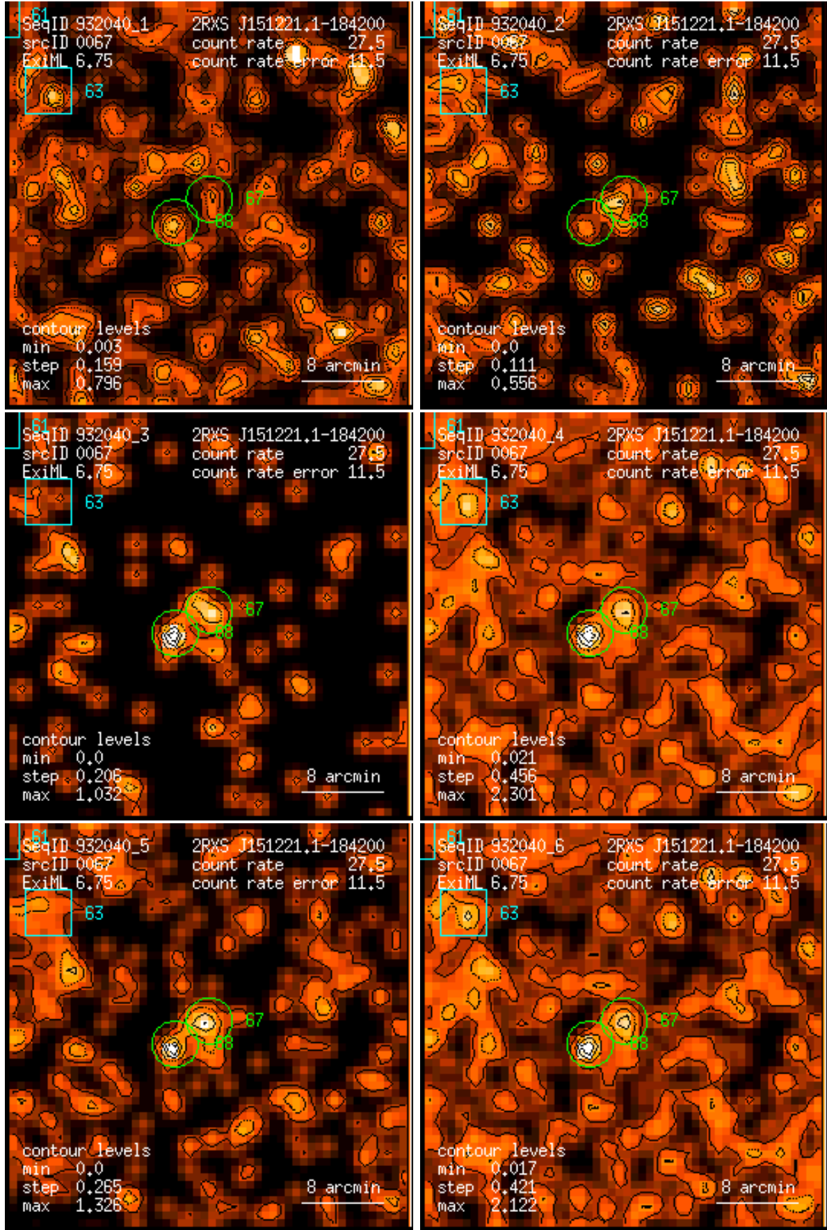
Figure 67: RASS 932040: detection 0067: band rate images, Gaussian filter: (1) PSPC channels 11 – 41, (2) 52 – 90, (3) 91 – 201, (4) 11 – 235, (5) 52 – 201, (6) 11 – 201. Broad band rates in counts/ks. Band rate contour levels in counts/ks/arcmin 2 .
