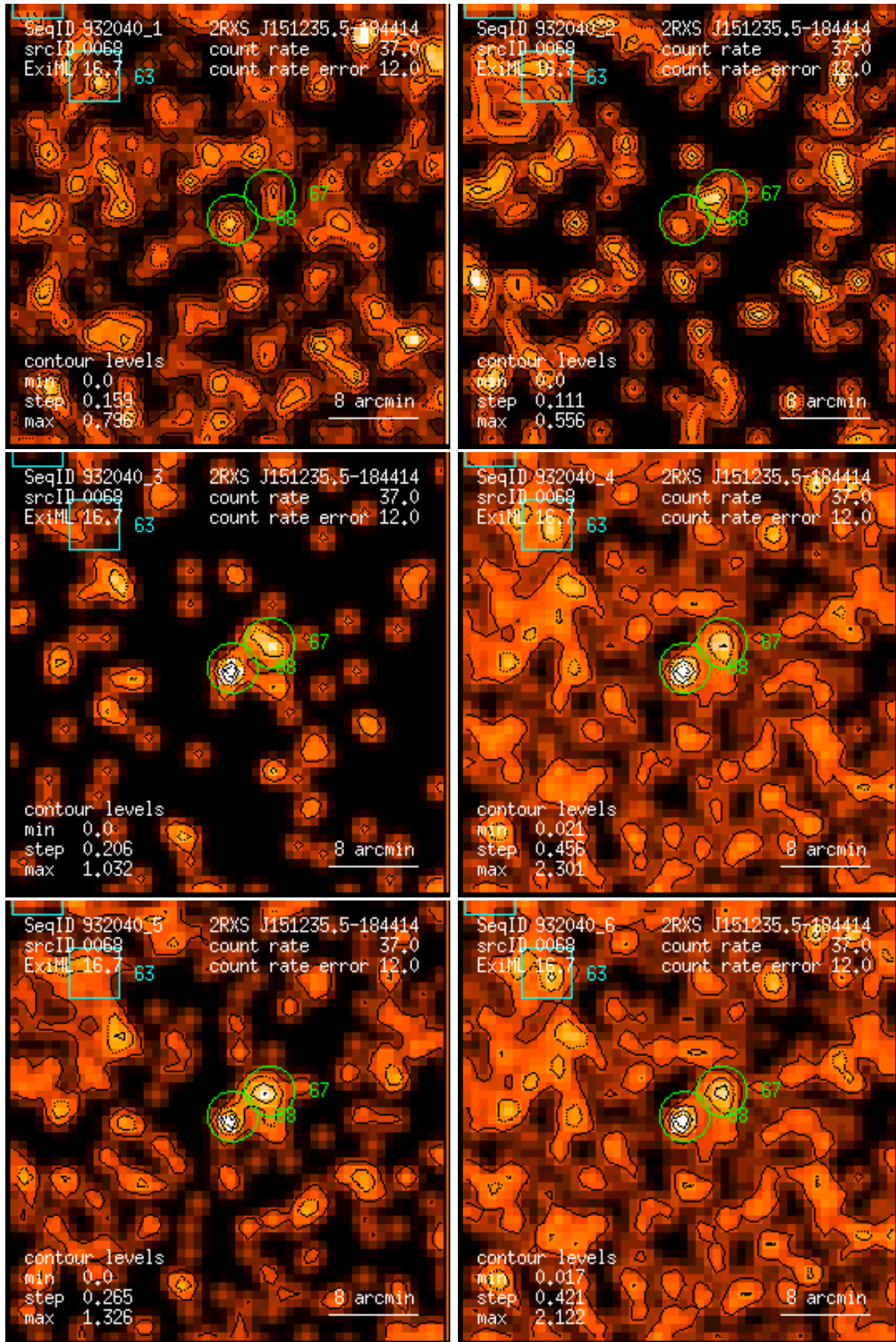
Figure 68: RASS 932040: detection 0068: band rate images, Gaussian filter: (1) PSPC channels 11 – 41, (2) 52 – 90, (3) 91 – 201, (4) 11 – 235, (5) 52 – 201, (6) 11 – 201. Broad band rates in counts/ks. Band rate contour levels in counts/ks/arcmin 2 .
