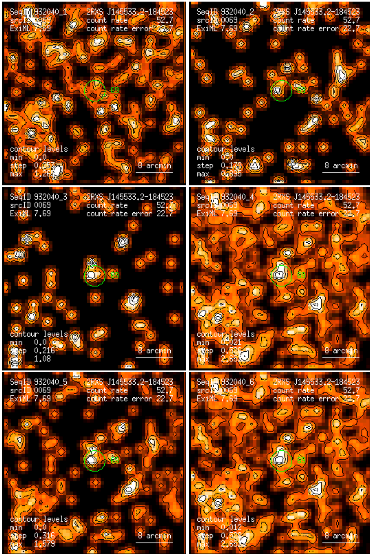
Figure 69: RASS 932040: detection 0069: band rate images, Gaussian filter: (1) PSPC channels 11 – 41, (2) 52 – 90, (3) 91 – 201, (4) 11 – 235, (5) 52 – 201, (6) 11 – 201. Broad band rates in counts/ks. Band rate contour levels in counts/ks/arcmin 2 .
