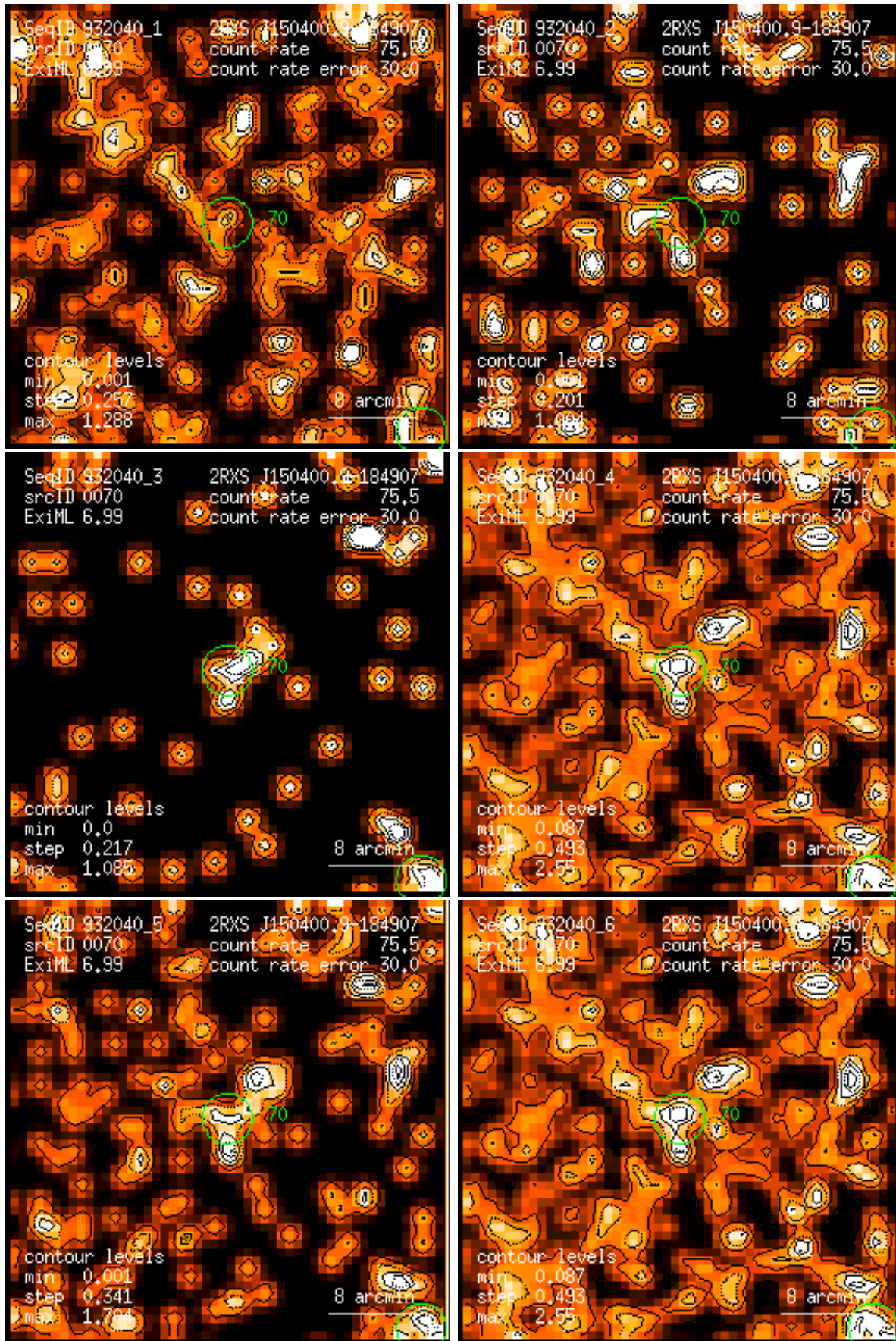
Figure 70: RASS 932040: detection 0070: band rate images, Gaussian filter: (1) PSPC channels 11 – 41, (2) 52 – 90, (3) 91 – 201, (4) 11 – 235, (5) 52 – 201, (6) 11 – 201. Broad band rates in counts/ks. Band rate contour levels in counts/ks/arcmin 2 .
