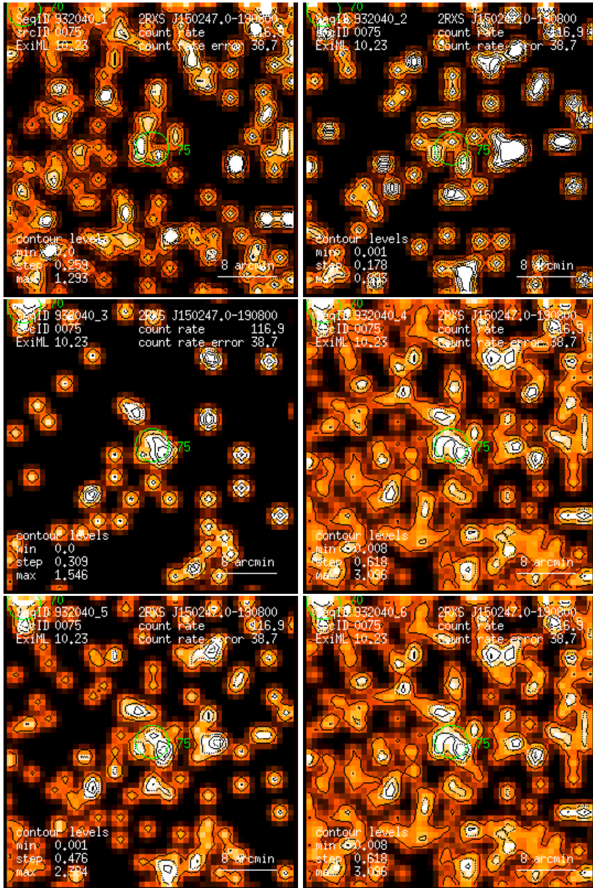
Figure 75: RASS 932040: detection 0075: band rate images, Gaussian filter: (1) PSPC channels 11 – 41, (2) 52 – 90, (3) 91 – 201, (4) 11 – 235, (5) 52 – 201, (6) 11 – 201. Broad band rates in counts/ks. Band rate contour levels in counts/ks/arcmin 2 .
