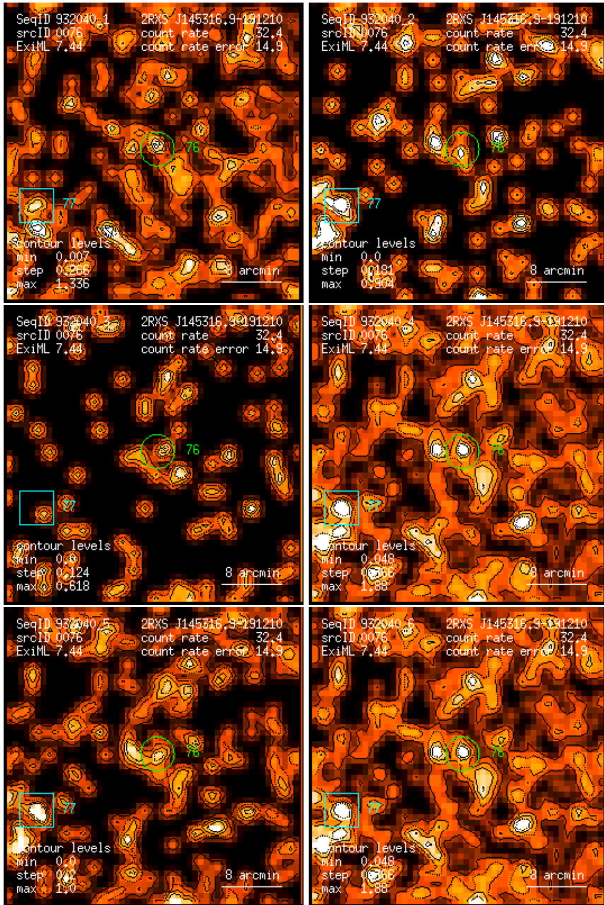
Figure 76: RASS 932040: detection 0076: band rate images, Gaussian filter: (1) PSPC channels 11 – 41, (2) 52 – 90, (3) 91 – 201, (4) 11 – 235, (5) 52 – 201, (6) 11 – 201. Broad band rates in counts/ks. Band rate contour levels in counts/ks/arcmin 2 .
